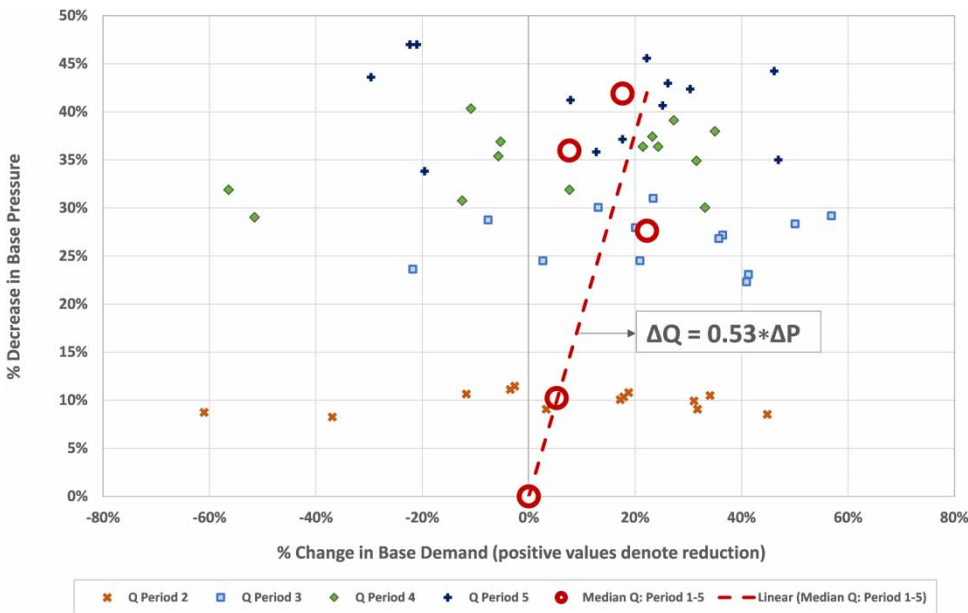
Figure 3 | Change in pressure versus change in consumer demand for DMA1.
