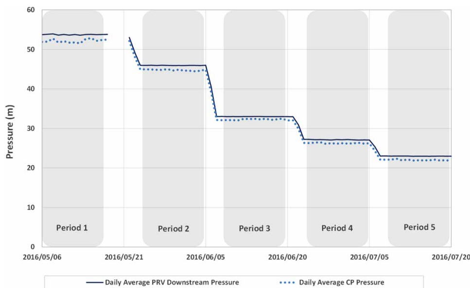
Figure 1 | DMA1 time series pressure profile.
