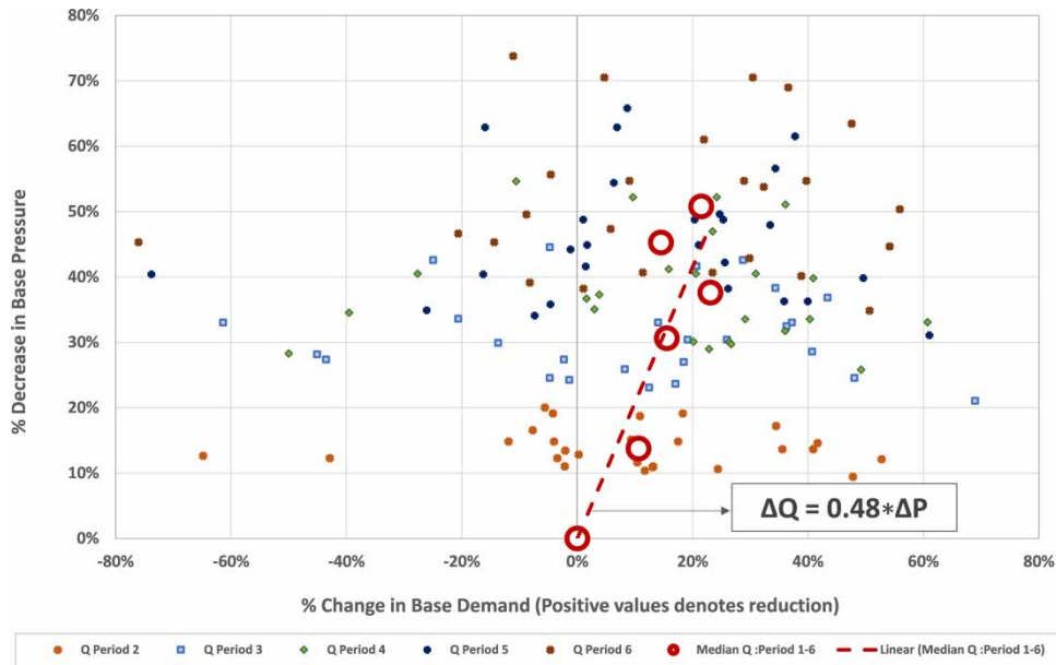
Figure 4 | Change in pressure versus change in consumer demand for DMA2.
