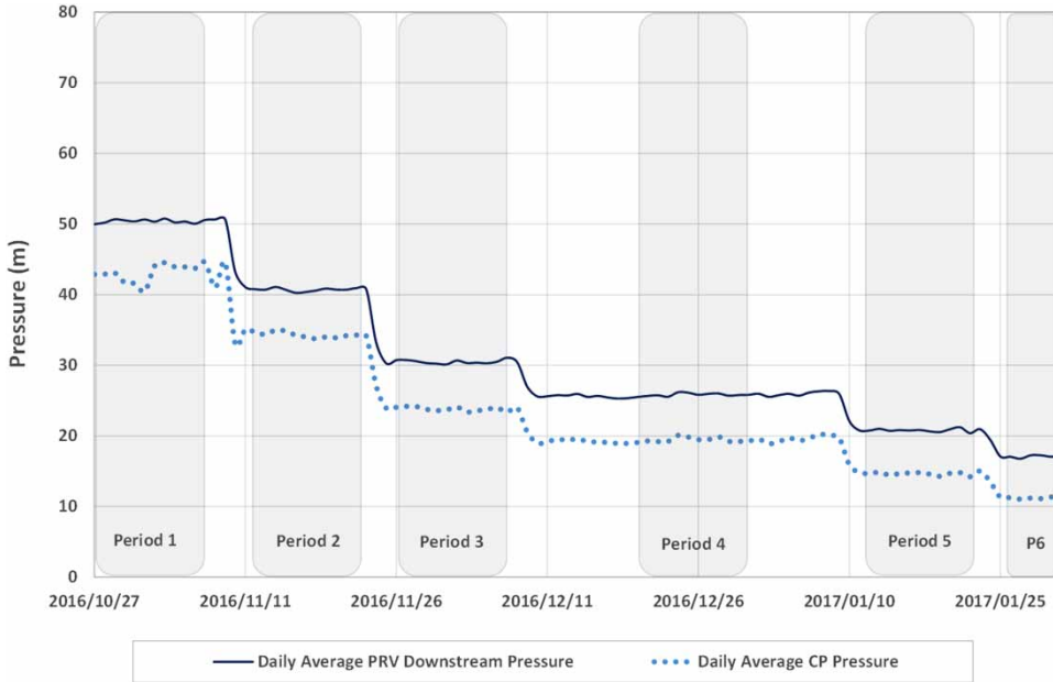
Figure 2 | DMA2 time series pressure profile.
