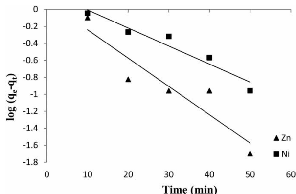
Figure 9 | Pseudo-first-order kinetics graph for Zn 2+ and Ni 2+ adsorption composite adsorbent. Initial Zn 2+ concentration of 30 ± 2 mg/L, initial Ni 2+ concentration of 25 ± 2 mg/L, shaking rate of 110 rpm, contact time of (10–60 min), and adsorbent dosage of 10 g/L.
