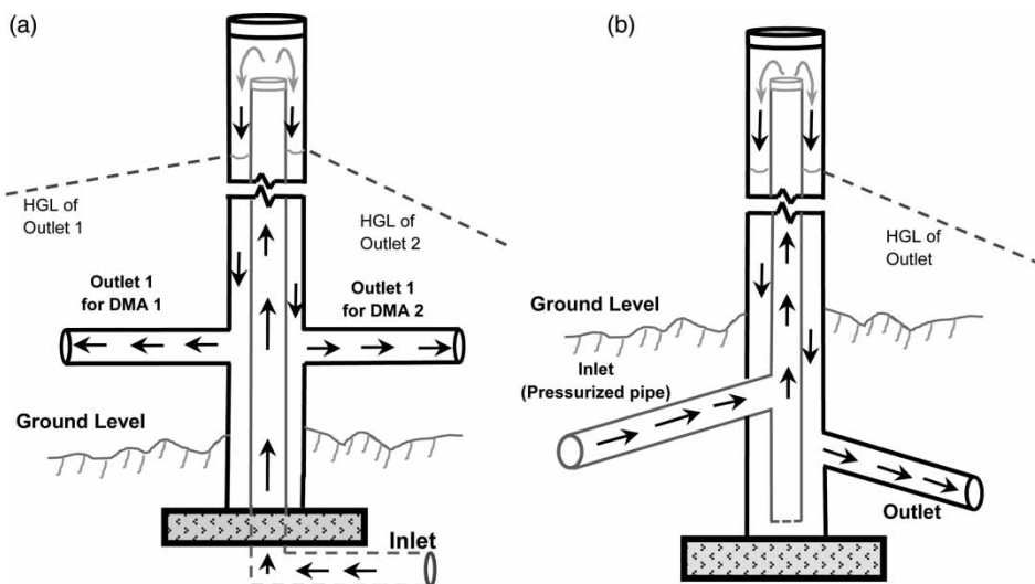
Figure 3 | (a) Shaft for distribution. (b) Shaft for transmission main.
