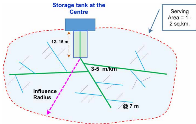
Figure 1 | Influence zone of the storage tank.
