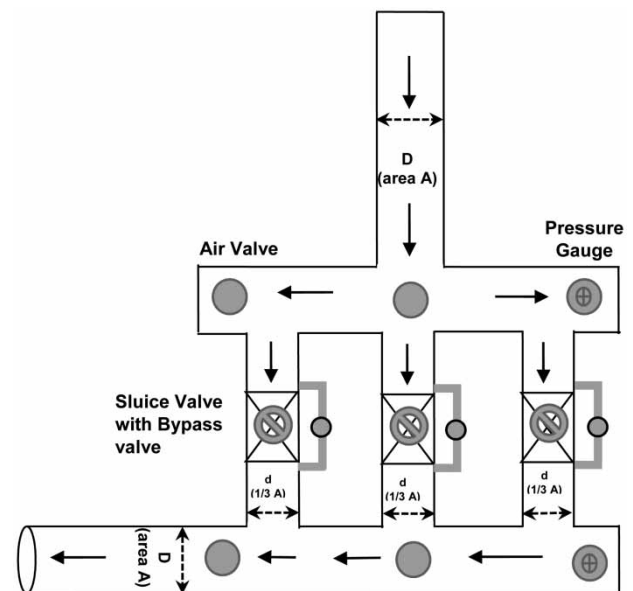
Figure 4 | Manifold system for stage-wise control of the flows in the system ( D is the internal diameter of the inlet/outlet pipe and A is the internal area of inlet/outlet pipe, d is the internal diameter of the small pipes having area of 1/3 A ).
