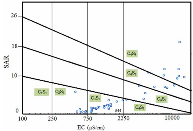
Figure 4 | Wilcox diagram (USSS classification) of the Marvdasht groundwater.
