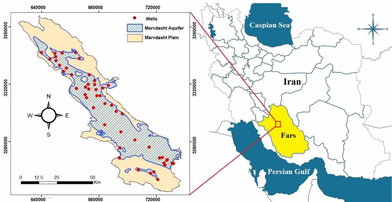
Figure 1 | Study area in Fars Province, Iran and the locations of sample sites.
