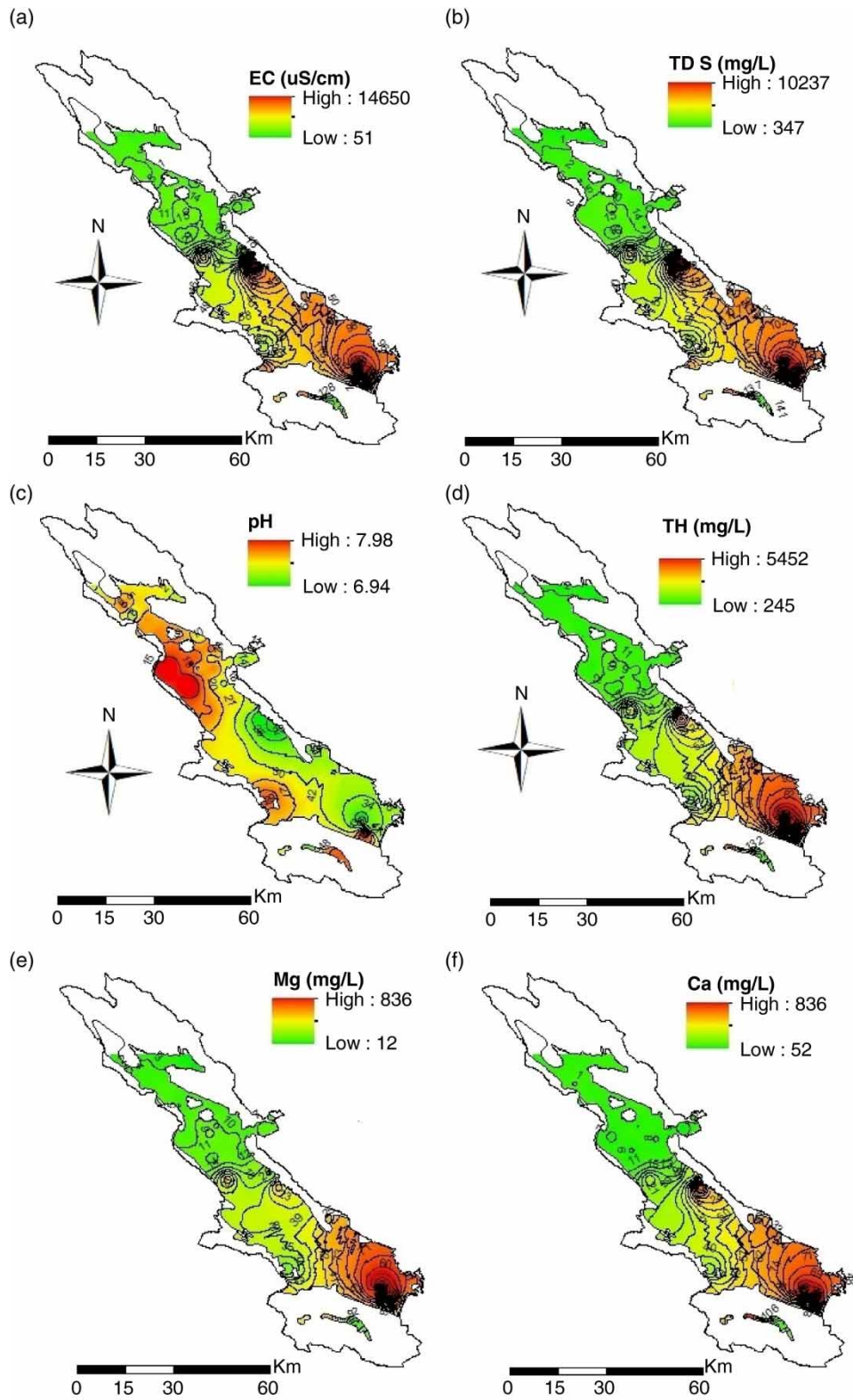
Figure 8 | Maps of Marvdasht groundwater quality parameters. (Continued.)
