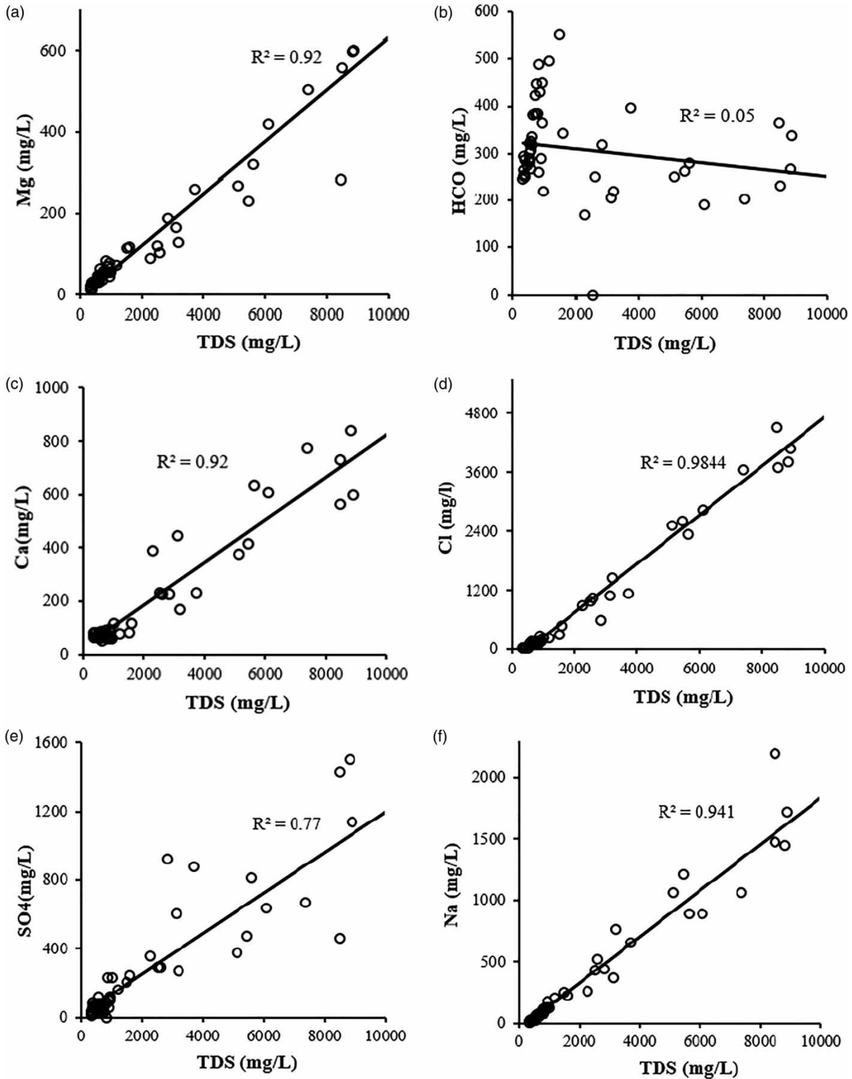
Figure 5 | Combined diagrams of various geochemical processes affecting TDS of Marvdasht groundwater.
