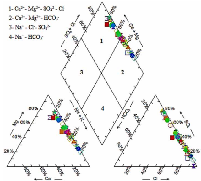
Figure 3 | Piper diagram of the Marvdasht groundwater.
