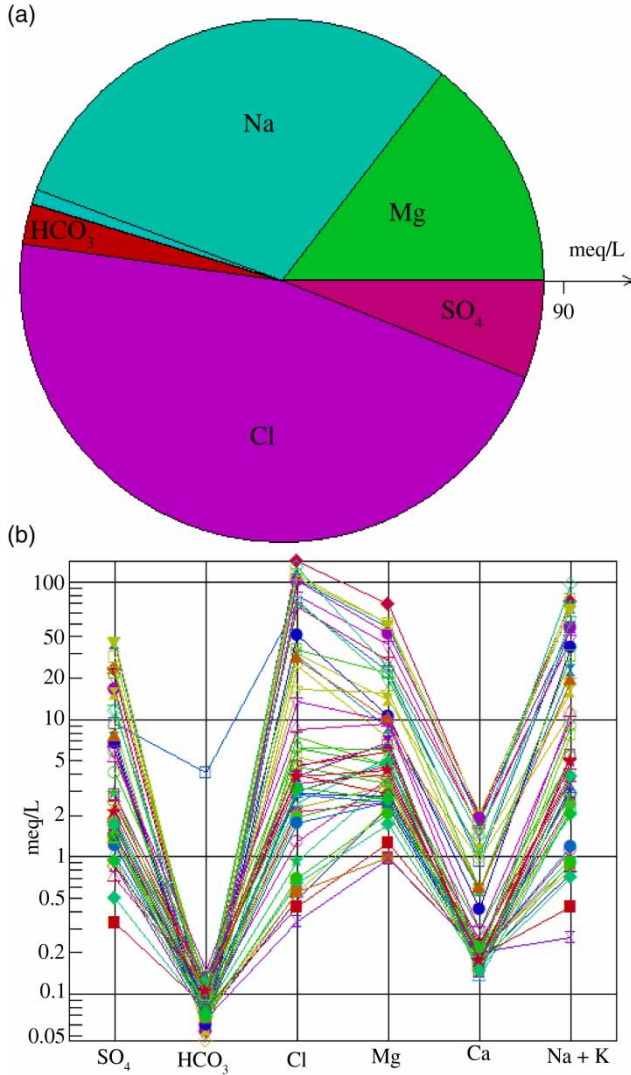
Figure 2 | Pie diagram (a) and Schoeller diagram (b).
