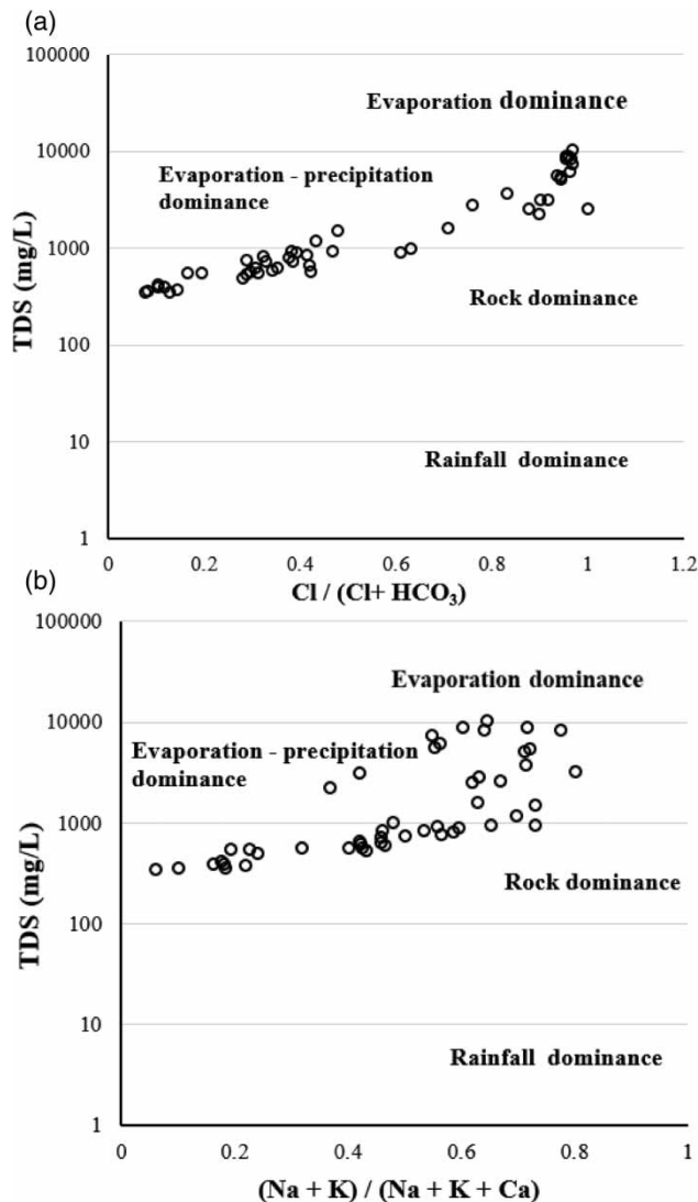
Figure 7 | Gibbs diagram of the Marvdasht aquifer.
