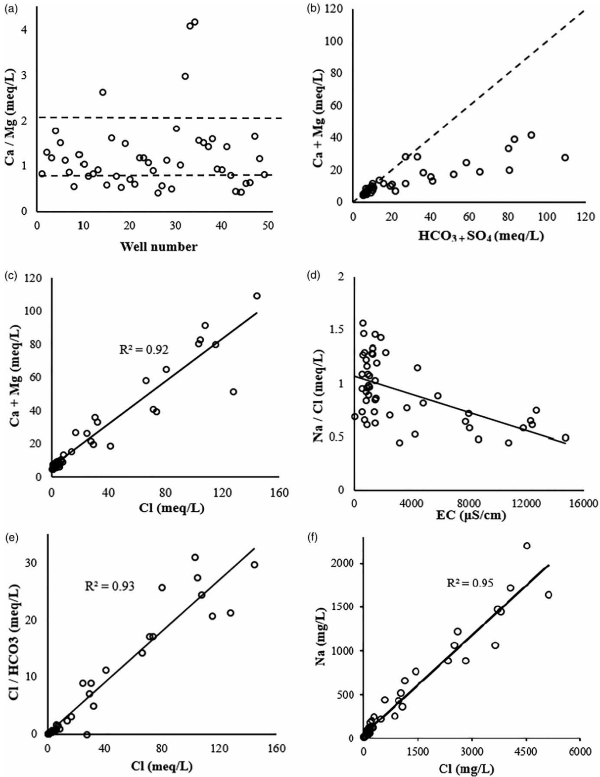
Figure 6 | Ionic ratio in Marvdasht groundwater.
