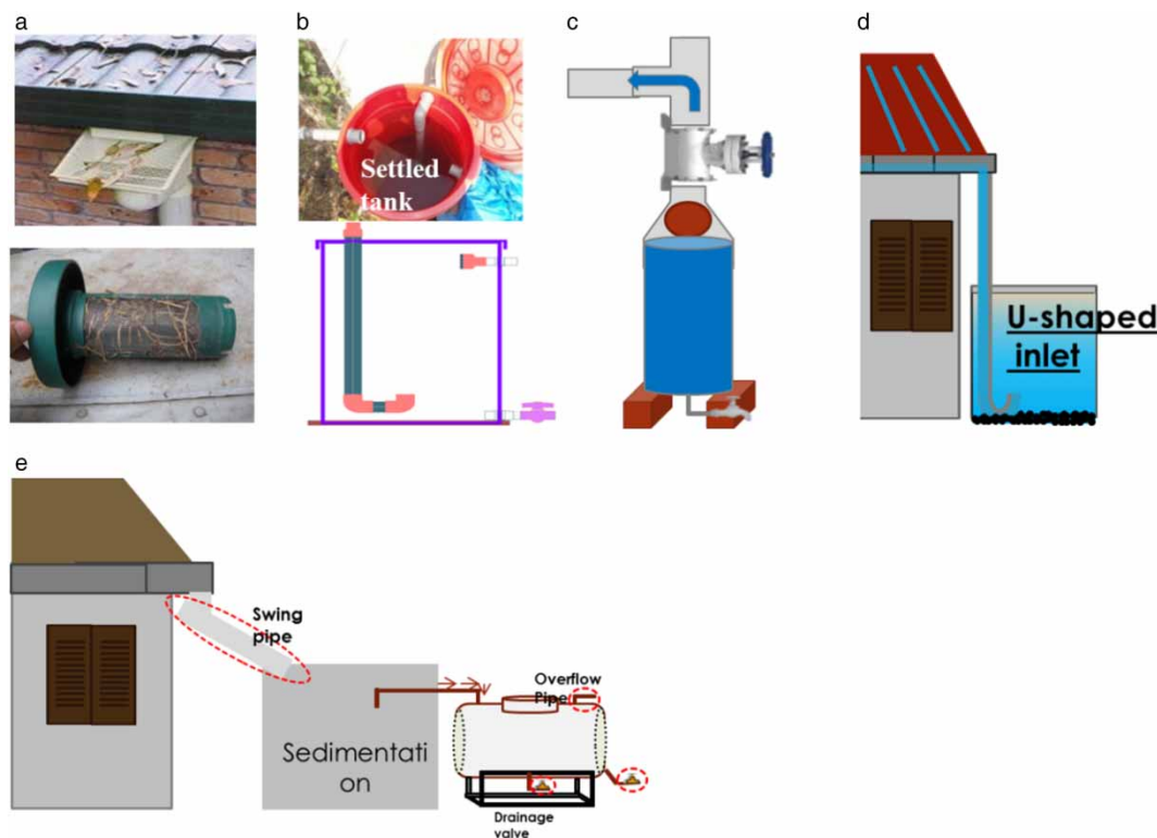
Figure 3 | Technologies to improve rainwater quality: (a) filter; (b) sedimentation; (c) first flush; (d) calm-inlet; (e) swing pipe.
