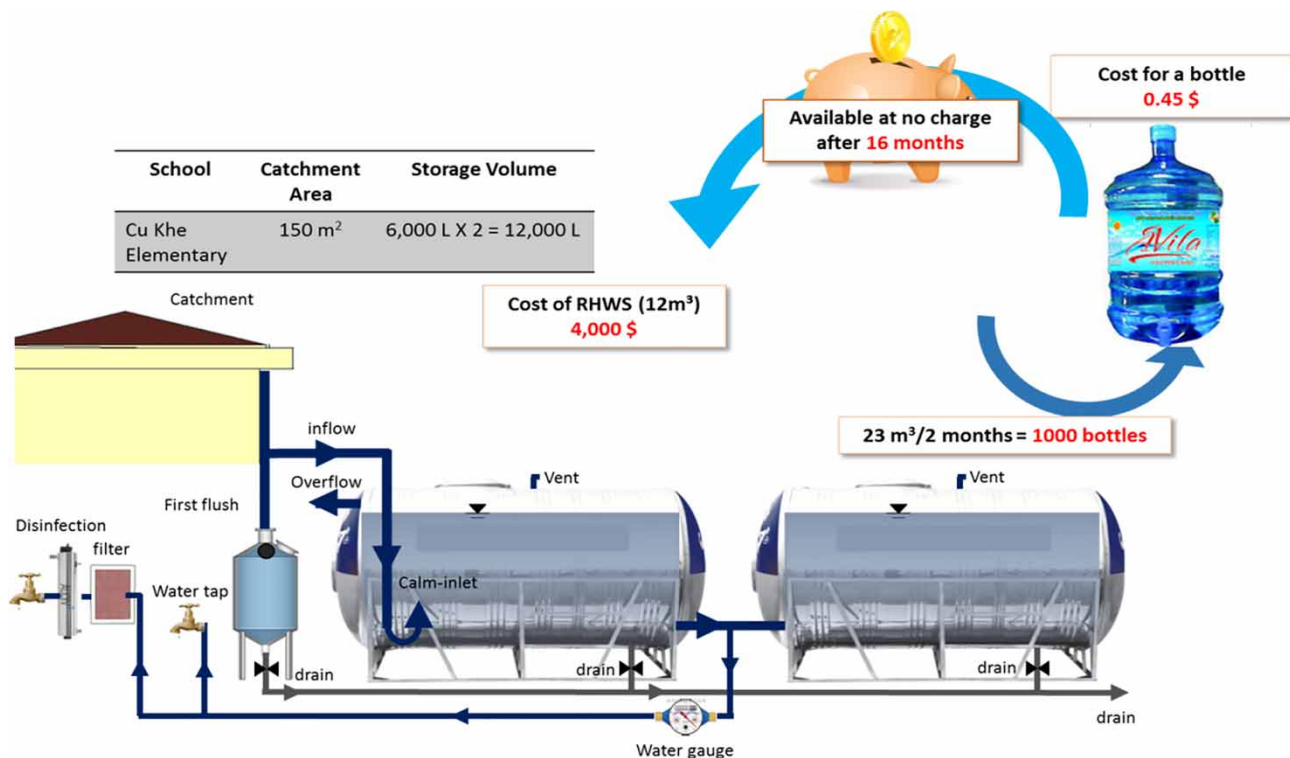
Figure 4 | RWH system in Cukhe kindergarten.
