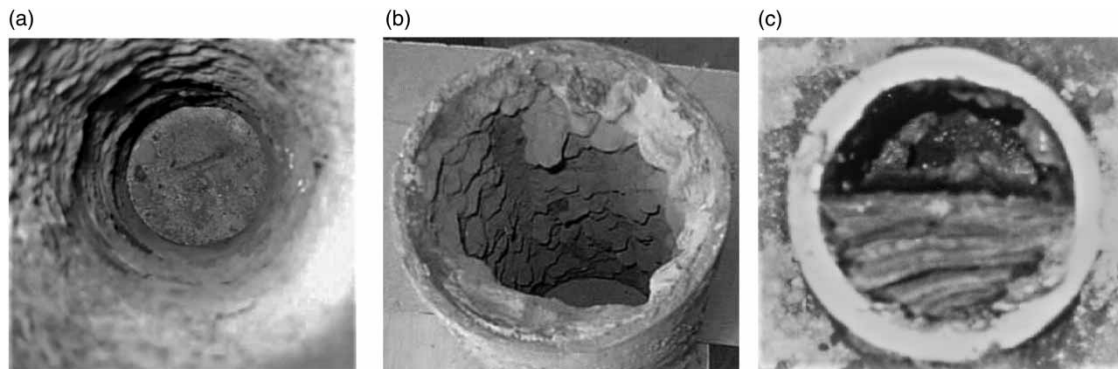
Figure 1 | Typical pipe wall build-up: (a) evenly distributed roughness; (b) unevenly distributed roughness; and (c) sediment settling. Samples from Tallinn WDS ( Kändler 2002 ).
