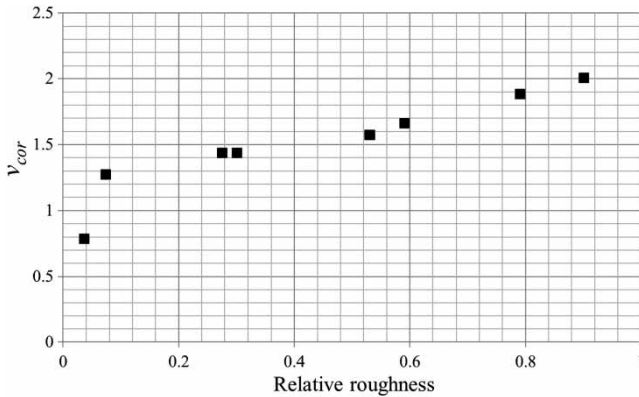
Figure 7 | Dependence between the velocity correction coefficient and the relative roughness (type 2, D = 100 mm and D = 200 mm).
