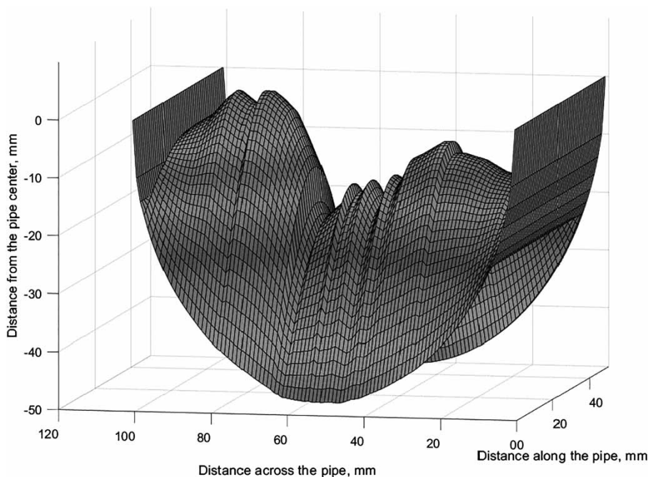
Figure 2 | 3D visualization of a random surface pattern.
