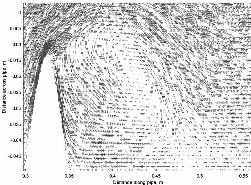
Figure 6 | Eddy convections near the roughness elements.
