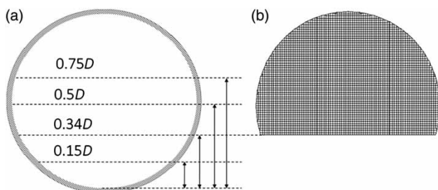
Figure 4 | (a) Numerically tested settlement heights 0.15D, 0.34D, 0.5D and 0.75D as measured from the pipe invert and (b) computational domain cross-section of a pipe representing settlement height 0.34D.
