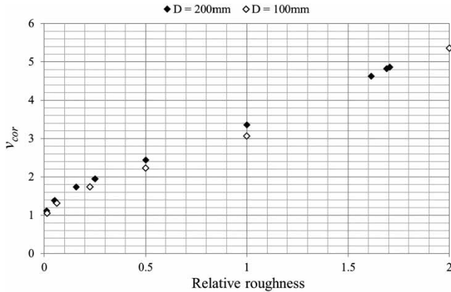
Figure 5 | Dependence between the velocity correction coefficient and the relative roughness (type 1).
