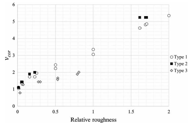
Figure 9 | Dependence between the velocity correction coefficient and the relative roughness (for all pipe types, D = 100 mm and D = 200 mm).
