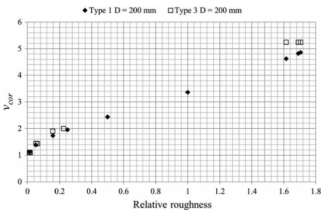
Figure 8 | Comparison of the dependence between the relative roughness and the velocity correction coefficient for type 1 and type 3 pipes.
