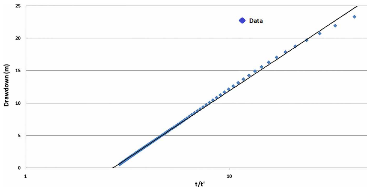
Figure 9 | Application of the recovery method on the second set of 5-min residual drawdown data on 15 April 2018.
