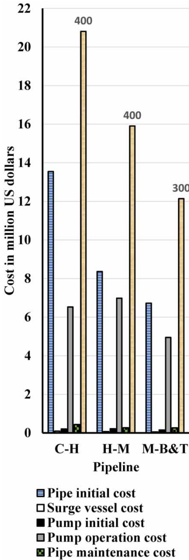
Figure 4 | Estimated cost of the actual project (with the used pipe diameter shown above the total cost bar in mm).
