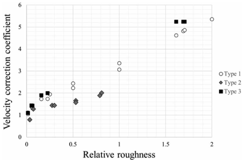
Figure 9 | Annus et al. (2020). Dependence between the velocity correction coefficient and the relative roughness (for all pipe types, D = 100 mm and D = 200 mm).
