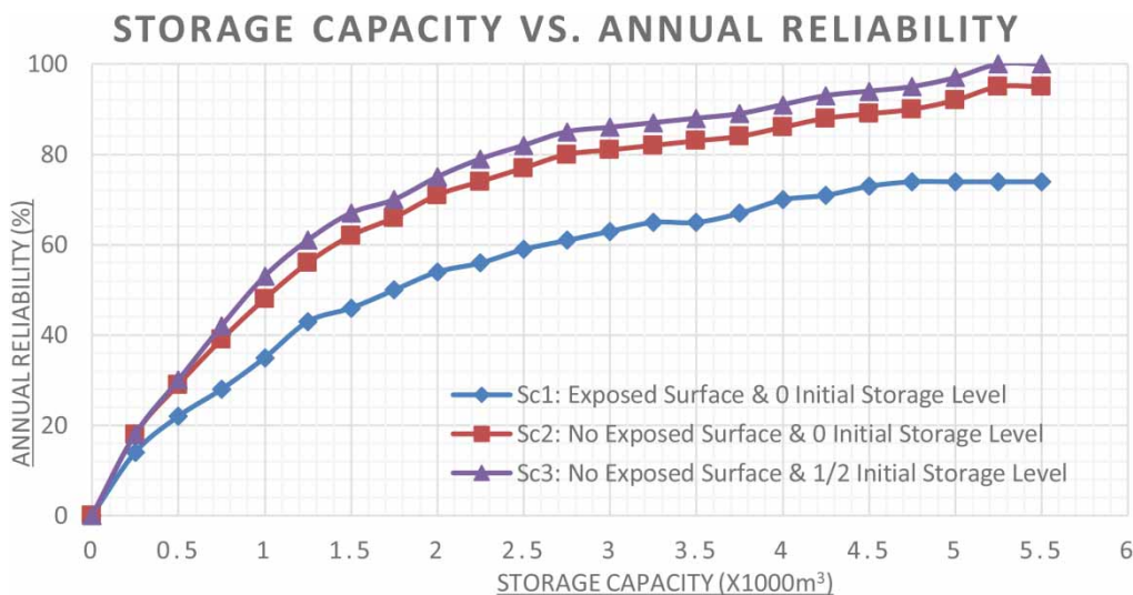
Figure 7 | Annual volumetric reliability of storage capacity.
