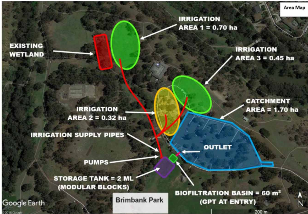
Figure 3 | Layout of the stormwater harvesting catchment, storage tank and other components.
