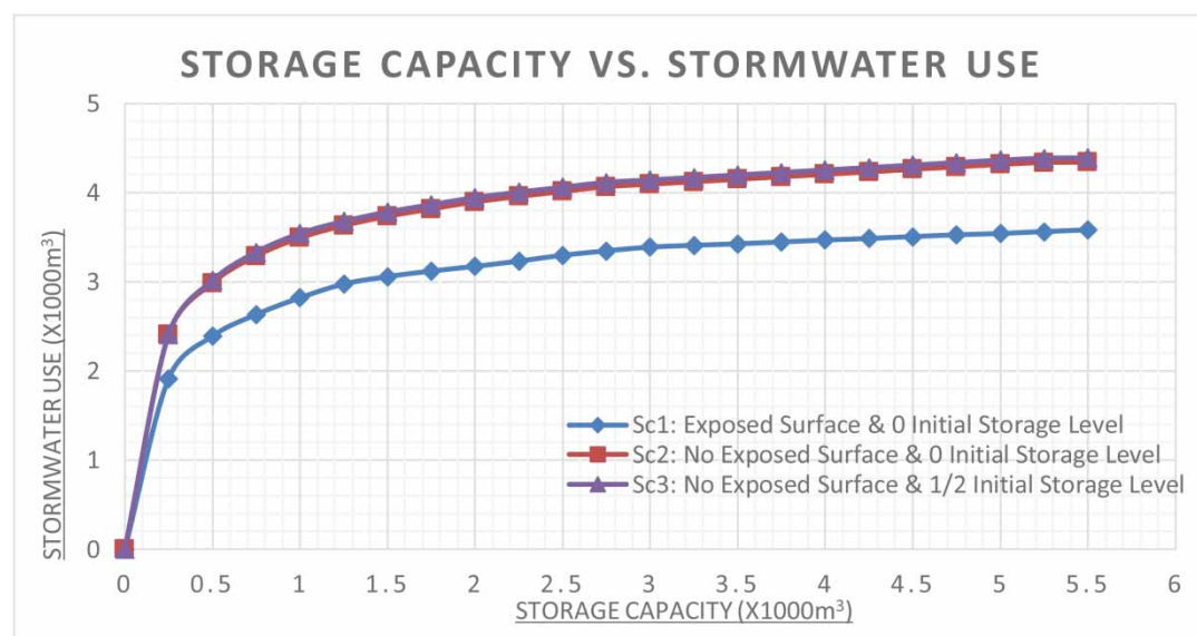
Figure 6 | Stormwater usage for irrigation and storage capacity.
