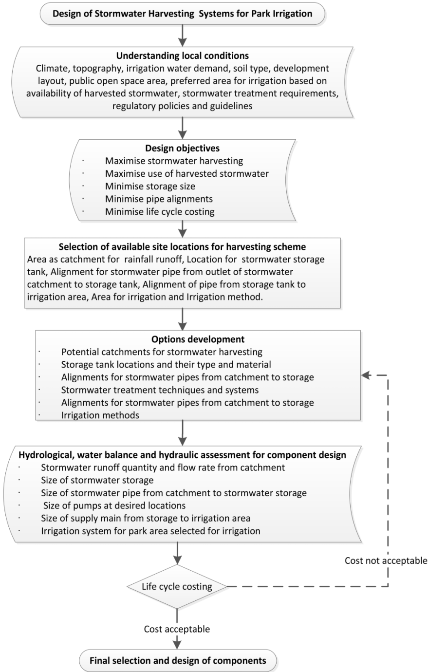
Figure 1 | Design methodology flowchart for stormwater harvesting scheme.
