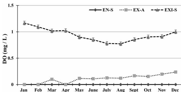
Figure 9 | Wastewater dissolved oxygen during 2019.
