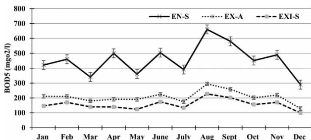
Figure 6 | Wastewater BOD 5 during 2019.
