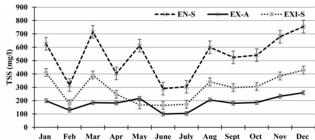
Figure 8 | Wastewater total suspended solids concentrations during 2019.
