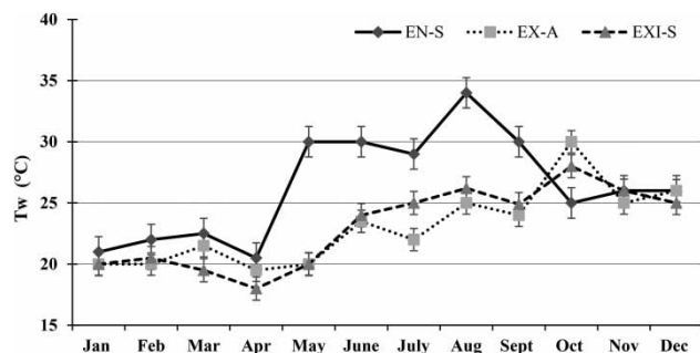
Figure 3 | Wastewater temperatures during 2019.
