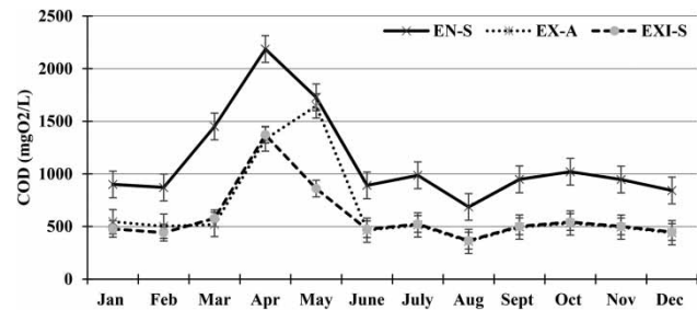
Figure 7 | Wastewater COD during 2019.
