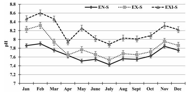
Figure 4 | Wastewater pH during 2019.
