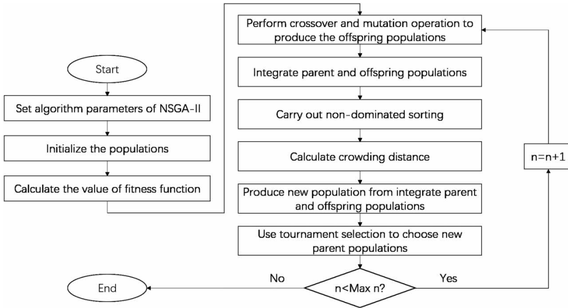
Figure 3 | The flowchart of NSGA-II.
