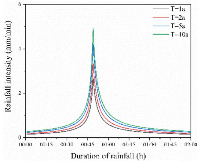
Figure 1 | Simulation results of Chicago rainfall pattern.
