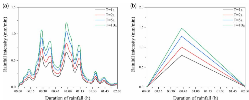
Figure 5 | Simulation results: (a) Pilgrim & Cordery rainfall pattern and (b) triangle rainfall pattern.
