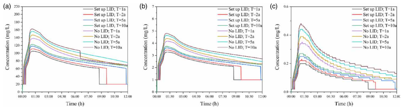
Figure 4 | Simulation results of infiltration gallery concentration: (a) simulation results of COD, (b) simulation results of TN and (c) simulation results of TP.
