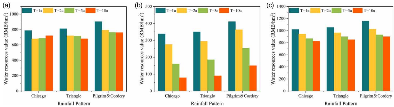
Figure 6 | Water resource value from different LID facilities under three rainfall patterns: (a) green roof, (b) infiltration pavement and (c) infiltration gallery.
