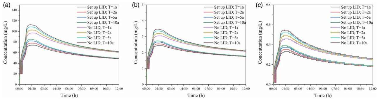
Figure 3 | Simulation results of infiltration pavement concentration: (a) simulation results of COD, (b) simulation results of TN and (c) simulation results of TP.
