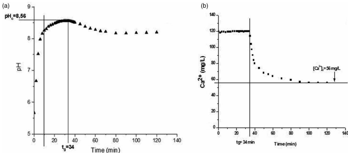
Figure 3 | Temporal evolution of CCP water pH (a) and concentration of Ca^{2+} (b) ( [Ca^{2+}]_0 = 120 \text{ mg}\cdot\text{L}^{-1} and T = 30^\circ\text{C} ).
