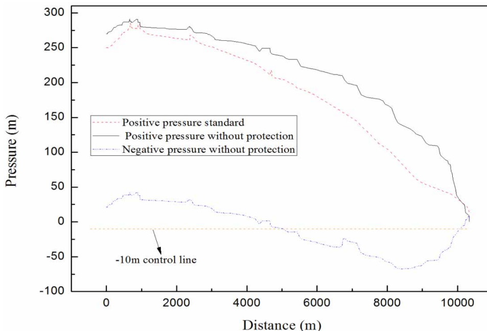
Figure 3 | Maximum and minimum pressure enveloping curves without any protection.
