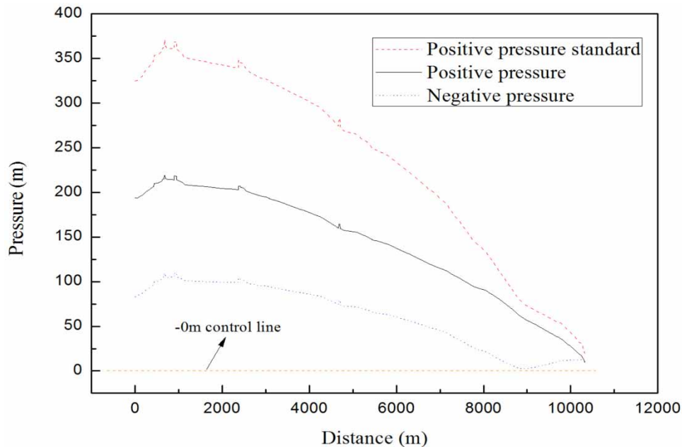
Figure 5 | The maximum and minimum enveloping curves of the AORV method.
