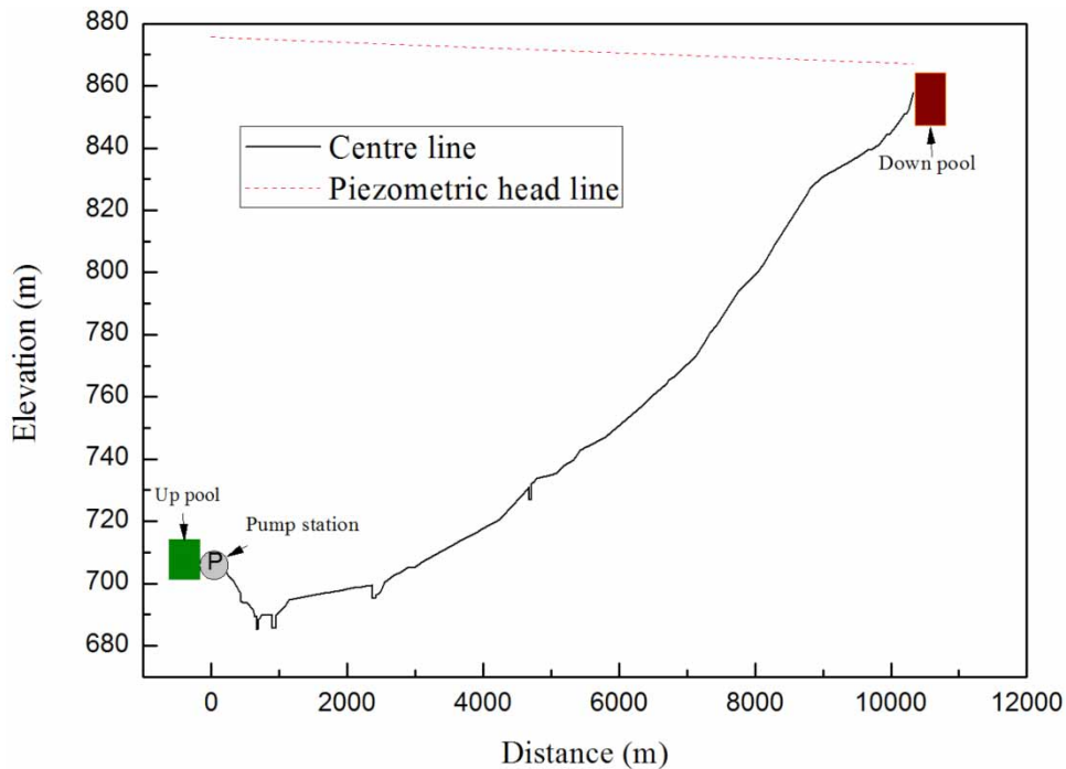
Figure 2 | Pipe center line, piezometric head line and schematic diagram of the water supply project.
