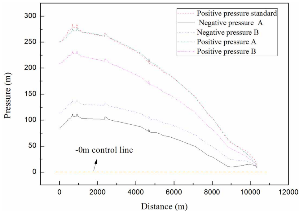
Figure 4 | Enveloping curves of pressures in methods A and B.
