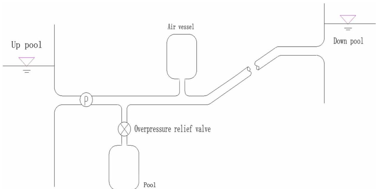
Figure 1 | Layout of water supply system with AORV combined method.
