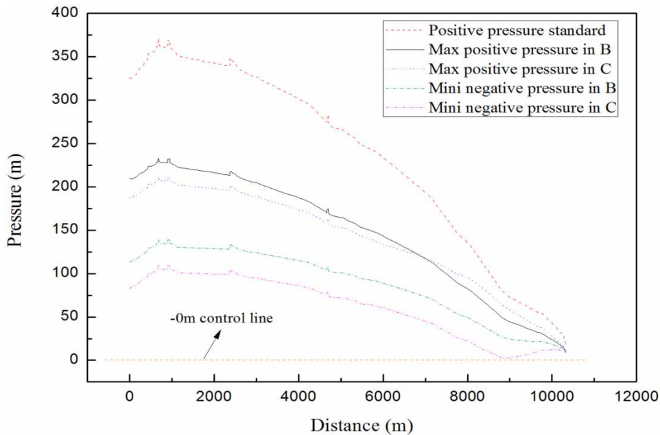
Figure 9 | The maximum and minimum pressure enveloping curves in different protective methods.
