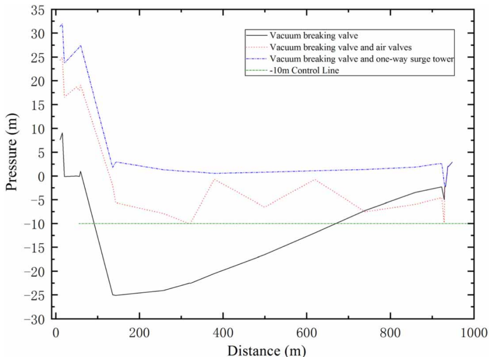
Figure 8 | Enveloping curves of minimum pressure in different protective schemes.
