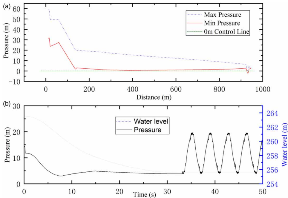
Figure 7 | (a) Enveloping curves of minimum pressure in the VBV and one-way surge tower scheme. (b) Variation process of bottom pressure and water level in the one-way surge tower.
