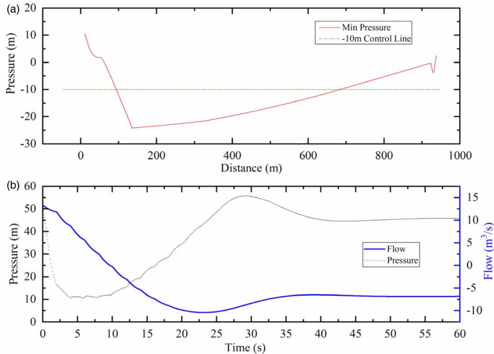
Figure 4 | (a) Minimum pressure enveloping curves without any protection and (b) variation pressure and flow after pump when pump trip happens.
