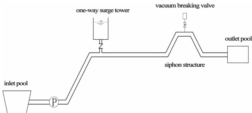
Figure 2 | Layout of the water supply system with the siphon structure in the VBV and one-way surge tower scheme.
