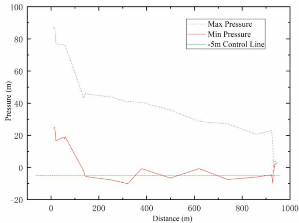
Figure 6 | Enveloping curves of minimum pressure in the VBV and air valve method.
