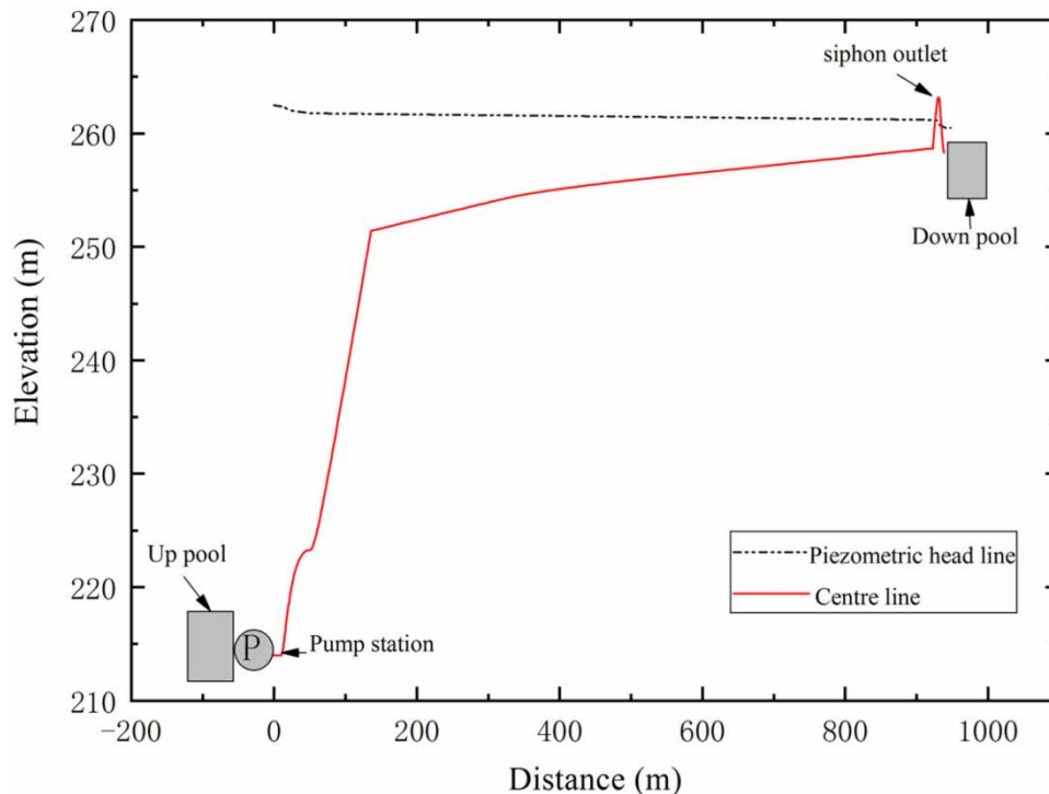
Figure 3 | Pipe centerline, piezometric headline and schematic diagram of the water supply project.
