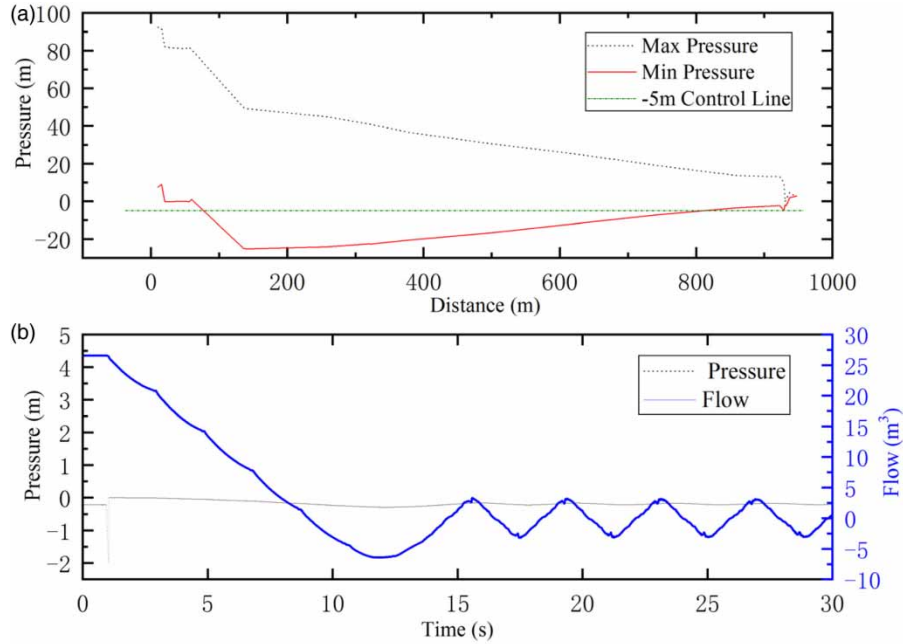
Figure 5 | (a) Enveloping curves of minimum pressure in the single VBV method and (b) variation pressure and flow at the siphon structure.
