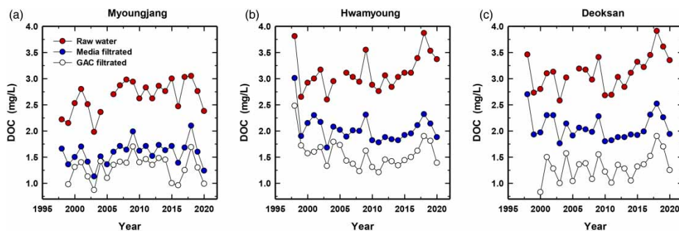
Figure 2 | Comparison of DOC concentration of raw water, media filtrated, and GAC filtrated over 1996–2020 at the Busan drinking water treatment facilities. Please refer to the online version of this paper to see this figure in colour: http://dx.doi.org/10.2166/aqua.2022.132 .
