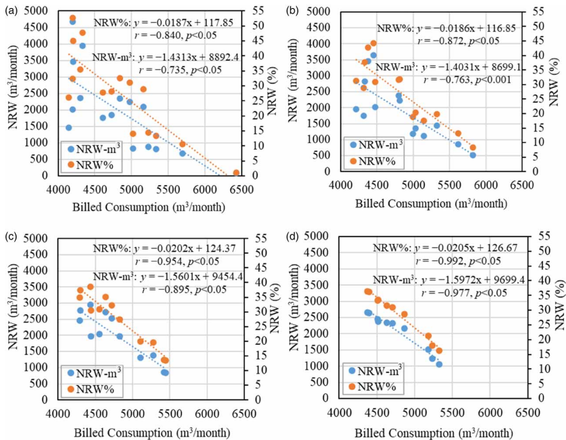
Figure 3 | Correlation between billed water consumption and \text{NRW-m}^3 or \text{NRW}\% in DMA-1. (a) Monthly; (b) 3-month moving averages (MA); (c) 5-month MA; and (d) 7-month MA. Data period: 16 months from January 2021 to May 2022 (excluding February 2021).
