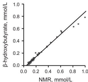
Figure 3. Comparison of circulating \beta -hydroxybutyrate quantification in an epidemiologic setting, using nuclear magnetic resonance (NMR) and an enzymatic method ( y -axis) ( n = 56 ) (105). The correlation coefficient is 0.98. See note on Figure 1 for the analytic correspondence.
