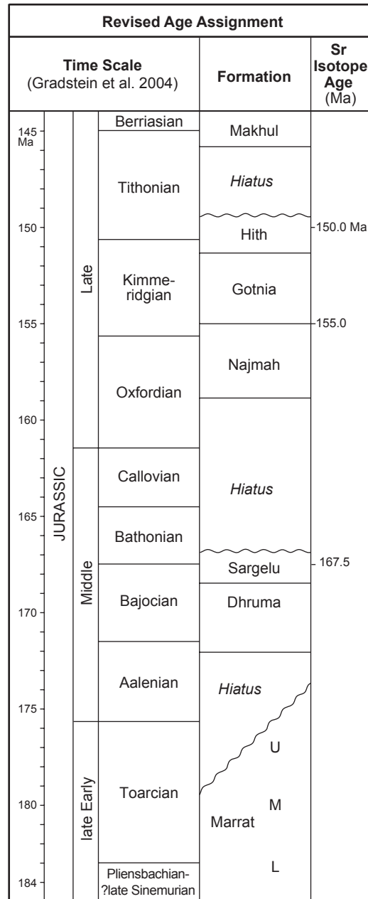
Figure: Jurassic type section of Kuwait based on the Minagish-27 well (Yousif and Nouman, 1997). On the right side, the revised ages of formations are shown using new biostratigraphic and strontium isotope data.
