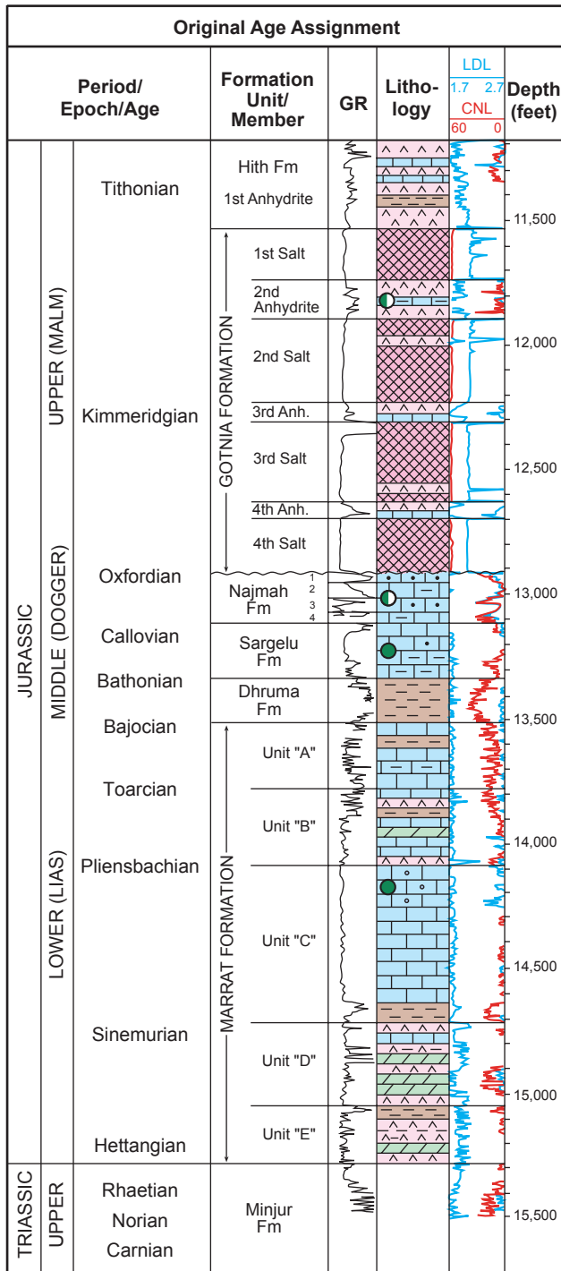
Figure: Jurassic type section of Kuwait based on the Minagish-27 well (Yousif and Nouman, 1997). On the right side, the revised ages of formations are shown using new biostratigraphic and strontium isotope data.
