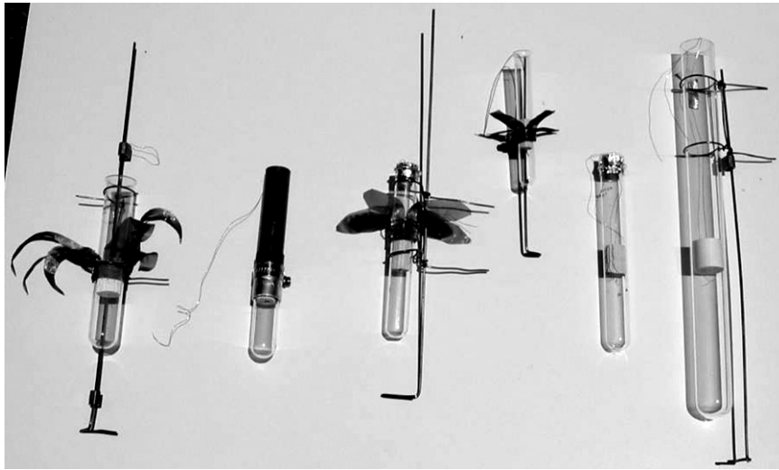
Fig. 4. Singing tube variants based on Penn State's "acoustic laser" [19], using different materials for stack components, tube dimensions, heat exchangers, etc. (Photo © M. Duffey)
