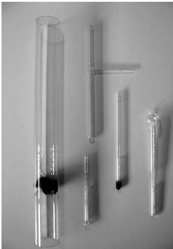
Fig. 3. Various singing tubes based on designs from the 19th- and 20th-century technical literature [15–18]. (Photo © M. Duffey) Most were built by master glassblower Gordon Good.
