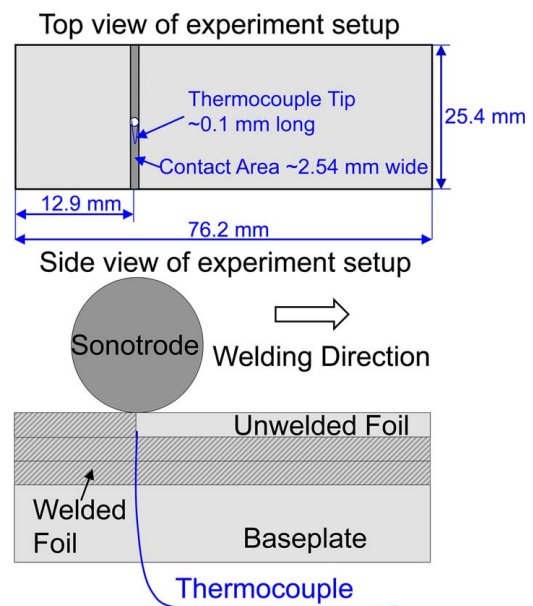
Fig. 1 Schematic of temperature measurement setup with the embedded thermocouple
