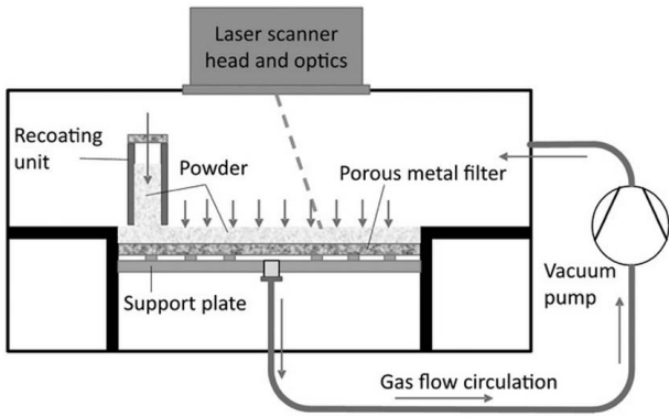
Fig. 2 Schematic of PBF prototype with the flow-assisted method [195]
