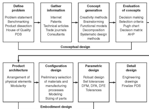
Fig. 2 Dieter and Schmidt’s first three phases of an engineering design process [50]. This model is referred to in this paper as the EDP process model.
