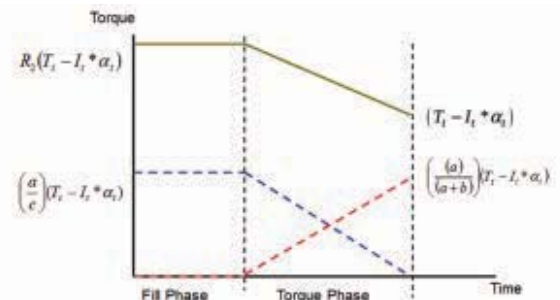
FIGURE 4 Diagram for clutch to clutch shift where R_2 is ratio, I_t is turbine inertia, T_t is turbine torque, \alpha_t is turbine acceleration, a, b, c are lever constants.
