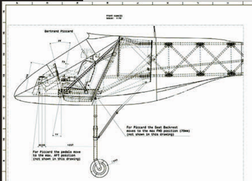
Drawings of the Solar Impulse 2's cockpit, and the finished structure. The entire space is 3.8 cubic meters.
