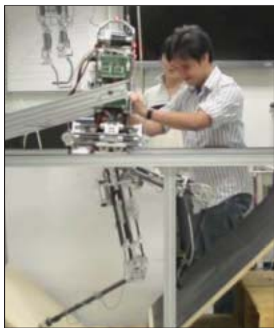
FIGURE 5. Multicontact control of the Hume biped standing on a V-shaped terrain while being disturbed by a student.
