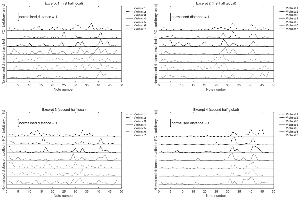
FIGURE 6. Normalized joint distance traveled in PC1 by note for each violinist in each cadential excerpt. For ease of visualization, each violinist's note-to-note distances were also normalized within each excerpt by dividing by the maximum distance traveled between two note onsets in an excerpt, but our statistical analysis was conducted on the values before this normalization.
