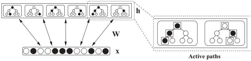
Figure 1: Illustration of a restricted Boltzmann forest for binary input vectors, where binary variables in the hidden layer are grouped in trees. When a hidden variable is inactive (white) or active (black), all hidden variables accordingly will be inactive in its left or right subtree. On the right (zoomed-in box), the variables in the active paths of two of the trees are identified.
