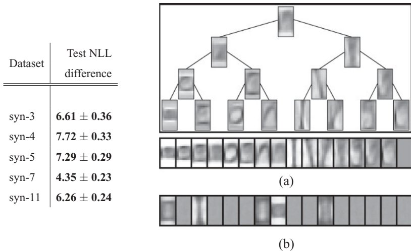
Figure 2: (Left) Comparison between using trees versus multinomial groups on five synthetic data sets (referred to as syn-T , where T \in \{3, 4, 5, 7, 11\} is the number of multinomial groups used to generate the data sets). The NLL difference is the NLL obtained using multinomial groups minus the NLL obtained using trees. (Right) Training optimization for a tree of hidden variables and a multinomial group. (a) Top: The illustration for a single-tree RBFforest of the weights W_{i,:} for each hidden variable. Bottom: The illustration of the summed weights W^T \mathbf{h} for all possible configurations of the hidden layer (i.e., the equivalent multinomial group weights). On the left of the tree root, weights captured different amounts of horizontal white backgrounds. On the right of the root, weights captured the structure of more vertically elongated characters. (b) Illustration of the weights learned using binary hidden variables forming a multinomial group. Most of them are still close to their initial near-zero value.
