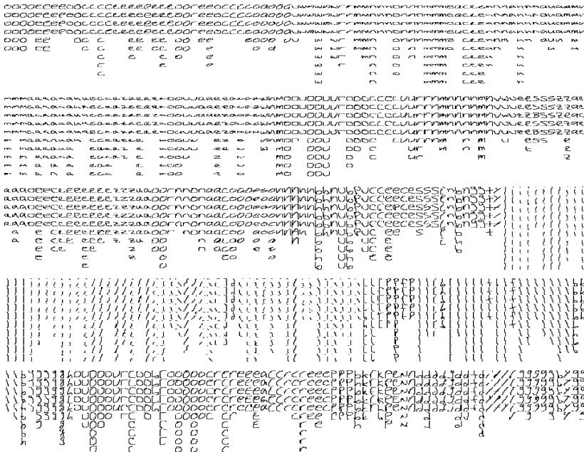
Figure 4: Visualization of 375 of the implicit mixture components (one per column) learned by the RBF on the ocr-letter data set.
