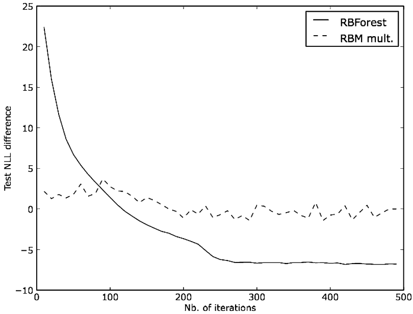
Figure 3: Learning curves for the RBForest and the RBM with multinomial groups on the syn-11 data set. To normalize the curves, the value of the test NLL at the end of the curve for the RBM with multinomial groups was subtracted to all test NLL errors. We see that RBForest is not simply converging faster but is actually finding a better minima than the RBM multinomial. The learning curve for RBM multinomial is also much less stable. Using a smaller learning rate (not shown here) gives a more stable behavior for RBM multinomial but worse performance.
