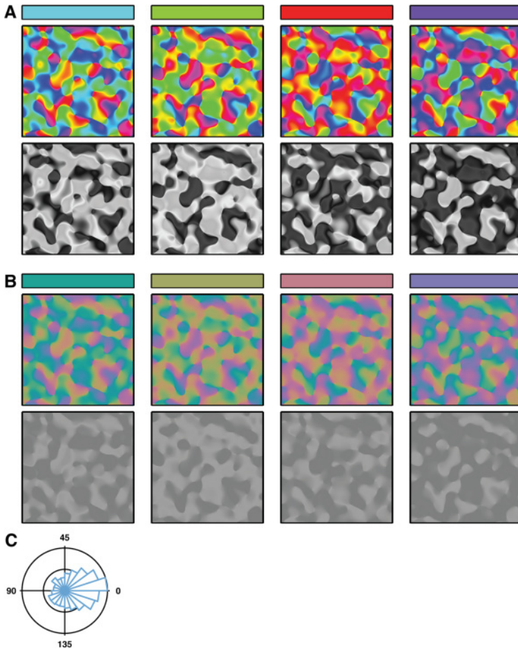
Figure 3: Perception of orientation preference maps with overrepresentation is highly dependent on the color mapping used to display them. An artificial orientation preference map with a single orientation overrepresented (identical map for all panels). In each column, a different hue is used to represent the overrepresented orientation, as indicated by the colored bars, and rows show preferred orientation and luminance. (A) Maps displayed with an HSV color mapping, with S = V = 100 . The perceived level of overrepresentation and more general map structure changes depending on which color is chosen to represent 0^\circ . (B) Maps displayed with an mHCL color mapping with C = 45 , L_0 = 60 , and m = 7 . A more accurate perception of map structure and overrepresentation level can be obtained when using an mHCL color mapping due to the minimal change in luminance between hues and the overall lower saturation. (C) Histogram of orientation preference in this map, showing the level of overrepresentation of the 0^\circ orientation.
