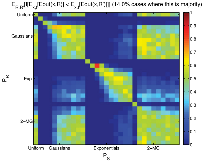
Figure 3: Summary of Monte Carlo simulation. The plot indicates, for each combination of probability distributions, \mathbb{E}_{R \sim P_R, R' \sim P_S} [\mathbb{I}[\mathbb{E}_{f, x \sim P_S} [\text{Eout}(x, R, f)] < \mathbb{E}_{f, x \sim P_S} [\text{Eout}(x, R', f)]]] .
