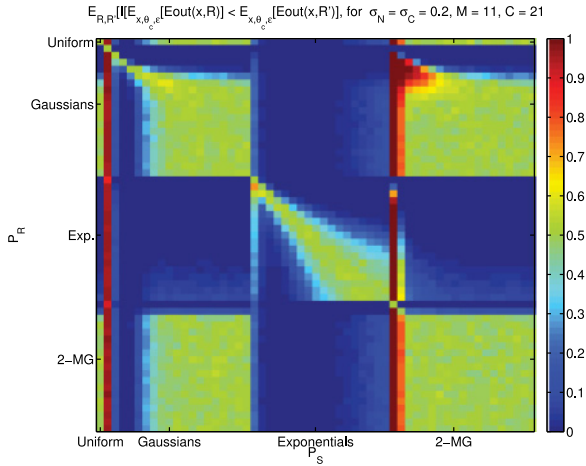
Figure 5: Monte Carlo simulation for \mathbb{E}_{R \sim P_R, R' \sim P_S} [I(\mathbb{E}_{x,\theta_c,\epsilon} [E_{out}(x,R)] < \mathbb{E}_{x,\theta_c,\epsilon} [E_{out}(x,R')])] , M = 11 , C = 21 , N = 500 , and \sigma_N = \sigma_C = 0.2 .
