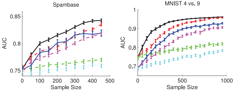
(a) AUC vs. sample size
