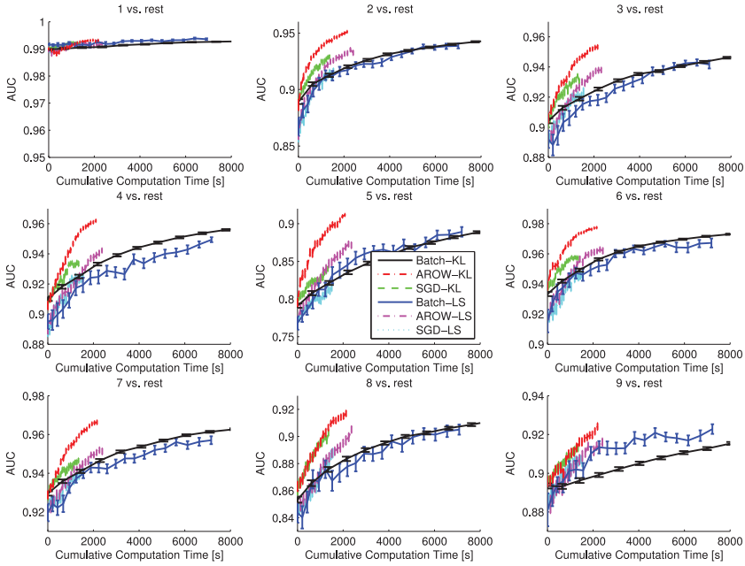
Figure 5: Computational time versus accuracy when a single digit is considered an inlier and the rest are considered outliers.
