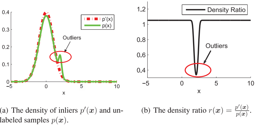
Figure 2: An example of density ratio-based outlier detection when the inlier and outlier distributions overlap. We see that (a) even when outliers occur in high-density areas, they can be (b) identified via the density ratio.
