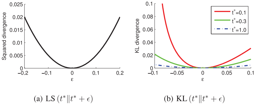
Figure 4: The squared loss LS(t^* || t^* + \epsilon) and the KL loss KL(t^* || t^* + \epsilon) for different values of t^* . The KL loss penalizes errors when t^* is small much more strongly.
