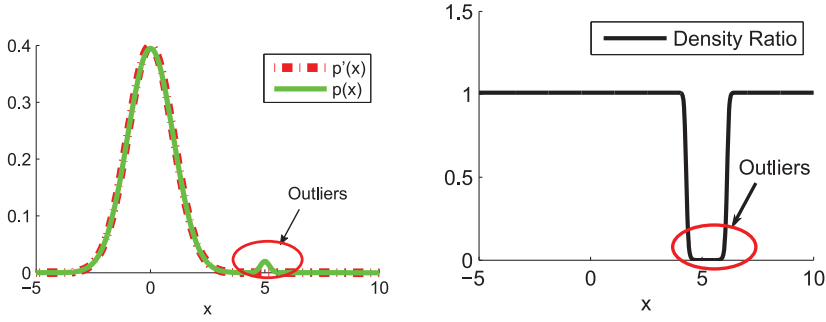
(b) The density ratio r(x) = \frac{p'(x)}{p(x)} .
