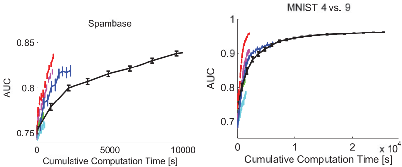
(c) AUC vs. computation time
