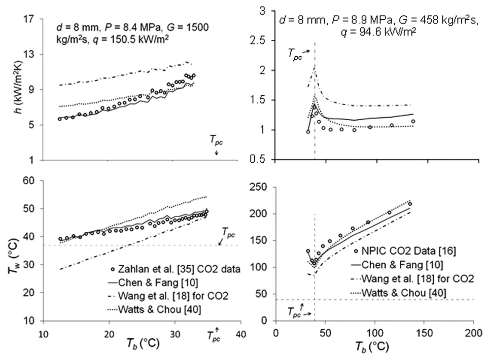
Fig. 3 Comparison of experimental h and T_w versus T_b and best-estimate circular tube correlations for CO 2
