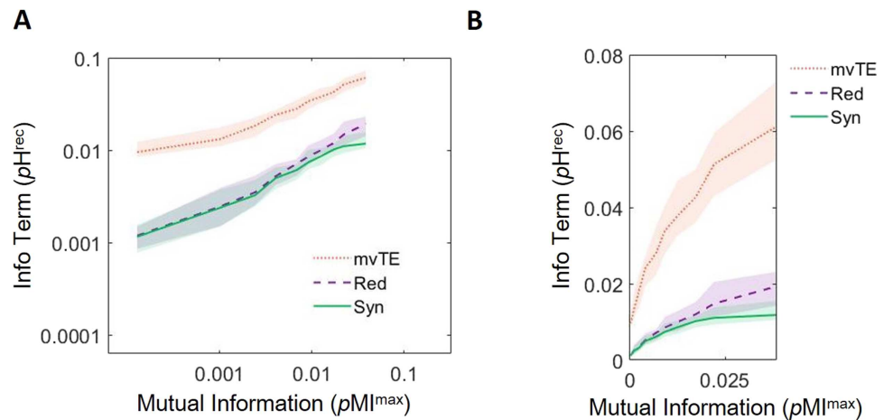
Figure 3. Growth of information transmission (mvTE) is greater than growth of redundancy over deciles of mutual information at synaptic timescales. (A) Multivariate transfer entropy (mvTE) and redundancy (Red) increase with mutual information. Synergy data is replotted here from Figure 2B for ease of comparison. (B) Same data as shown in A without log-scaling to show rapid growth of mvTE relative to redundancy. For all plots, lines depict medians and shaded regions depict 95% bootstrap confidence intervals around the median.
