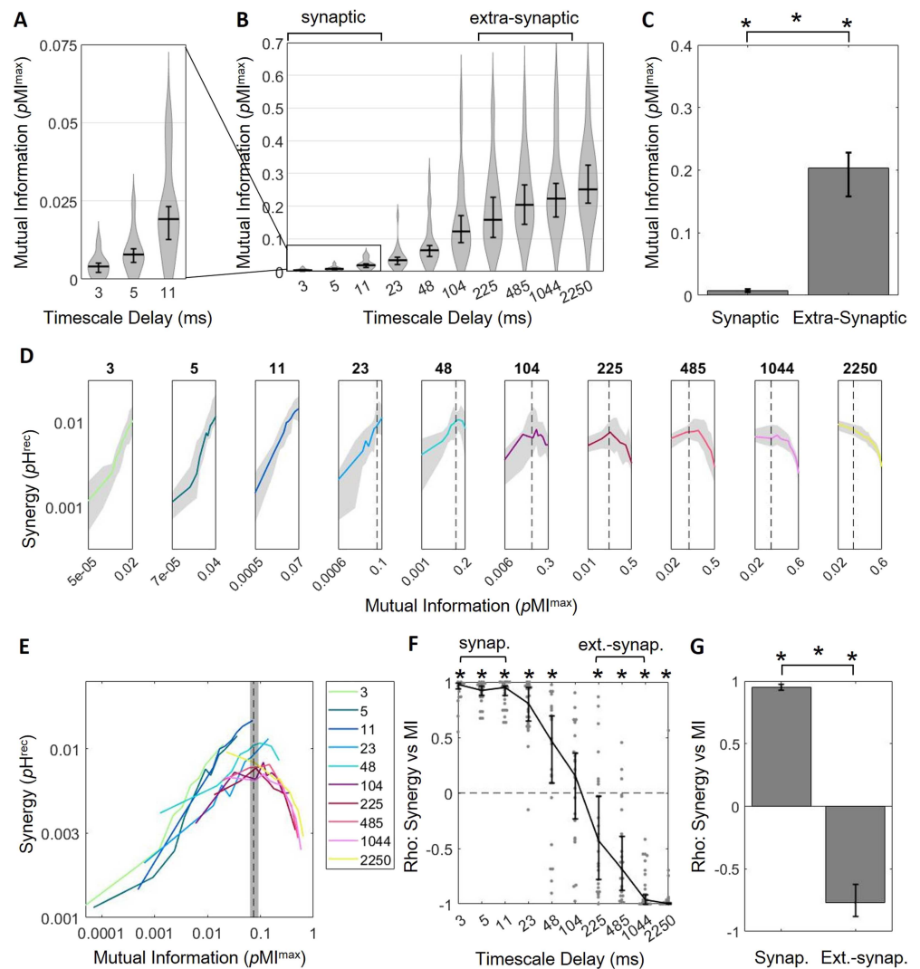
Figure 4. Greater correlated activity emerges at longer timescales with diminishing returns for synergistic processing. (A) Median mutual information increases across synaptic timescales. (B) Median mutual information continues to increase at extrasynaptic timescales. (C) Median mutual information is significantly larger at extrasynaptic timescales than at synaptic timescales. (D) Plotting synergy as a function of mutual information across timescales shows that the positive relationship between synergy and mutual information only exists at synaptic timescales where mutual information is relatively low. This relationship becomes negative at extrasynaptic timescales where mutual information is high. Note that mutual information, plotted along the x -axis, varies across subpanels. A dashed vertical line where mutual information is 0.07 is included to facilitate visual alignment across panels. (E) Curves from D are replotted on the same axes here to show the overall relationship between synergy and mutual information. (F) Spearman rank correlation coefficients of synergy versus mutual information for all networks across timescales show that synergy and mutual information are positively related at shorter timescales and negatively related at longer timescales. (G) Synergy and mutual information are significantly positively correlated at synaptic timescales and significantly negatively correlated at extrasynaptic timescales. For all plots shown above, bars/solid lines indicate medians, shaded regions/error bars depict 95% bootstrap confidence intervals around the median, and * indicates p < 0.05 .
