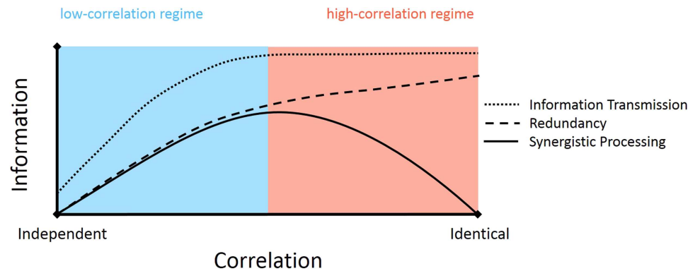
Figure 6. Neural computation can be expressed as a function of the correlation between inputs. When the correlation of inputs is low, synergistic processing benefits from increased correlation. In this regime, both information transmission and redundancy increase with greater correlation, but information transmission grows faster than redundancy effectively increasing the bandwidth available for synergistic processing. When the correlation of inputs is high, synergistic processing is hurt by increased correlation. In this regime, redundancy and not information transmission increases with greater correlation, reducing the bandwidth available for synergistic processing.
