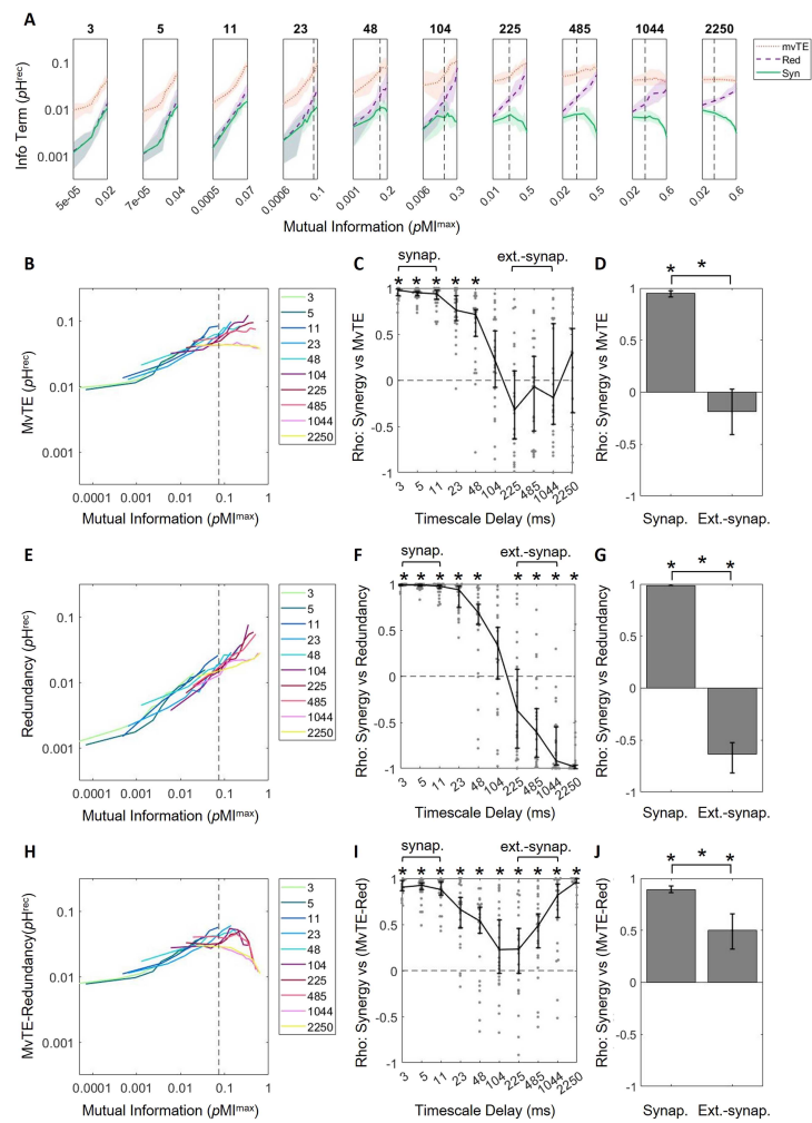
Figure 5. Redundancy encroaches upon multivariate transfer entropy at longer timescales, accounting for decreasing synergy at those timescales. (A) Log-scaled multivariate transfer entropy (mvTE), redundancy (Red), and synergy (Syn) versus mutual information, for all timescales. Growth of mvTE with respect to mutual information is steep at short timescales, but decreases across timescales. Redundancy grows with mutual information at all timescales. (B) MvTE curves in A plotted on the same axes. (C) Spearman rank correlation coefficients of synergy versus mvTE across timescales indicates that mvTE saturates at longer timescales. (D) Synergy and mvTE are significantly positively related at synaptic timescales, but not at extrasynaptic timescales. (E) Redundancy curves in A plotted on the same axes. (F) Spearman rank correlation coefficients of synergy versus redundancy across timescales shows how the two are positively related at shorter timescales and negatively related at longer timescales. (G) Synergy and redundancy are significantly positively related at synaptic timescales and significantly negatively related at extrasynaptic timescales. (H) Difference of MvTE and redundancy curves in A plotted on the same axes shows that the overall trend looks most similar to that of synergy versus mutual information in Figure 4E. (I) Spearman rank correlation coefficients of synergy versus mvTE redundancy across timescales shows that the two are positively related at all timescales. (J) Synergy and mvTE redundancy are significantly positively related at synaptic and extrasynaptic timescales. Synergy versus mutual information data has been replotted from Figure 4D here in A for ease of comparison. For all plots, solid/bold lines indicate medians and shaded regions/error bars depict 95% bootstrap confidence intervals around the median.
