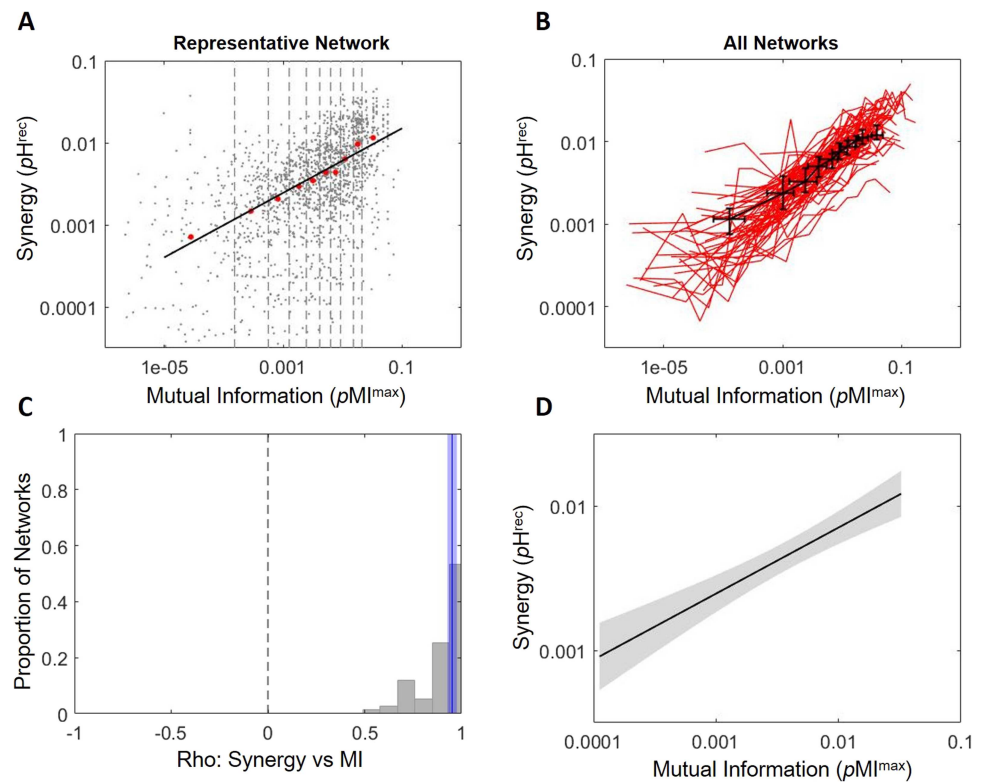
Figure 2. Increased correlated activity predicts greater synergistic processing at synaptic timescales. (A) Synergy plotted as a function of mutual information for a representative network shows a positive relationship. Gray dots indicate individual triads. Boundaries of deciles of mutual information are depicted via dashed lines. Median synergy for each decile (red dots) increased across deciles. The black line shows the linear least squares fit of the red dots ( \rho = 0.99 , slope = 0.39). (B) Synergy across mutual information deciles for all 75 synaptic timescale networks are shown as red lines. The median synergy and mutual information for each decile is shown by the black points with error bars indicating 95% bootstrap confidence intervals. (C) Histogram of Spearman rank correlation coefficients for synergy versus mutual information shown in B. A solid blue line marks the median correlation coefficient across the 75 networks, and the shaded region around the blue line shows the 95% bootstrap confidence interval around the median. (D) Average regression fit line across the 75 linear regressions of synergy versus mutual information indicates consistently positive relationship. Shaded region indicates the 95% confidence interval.
