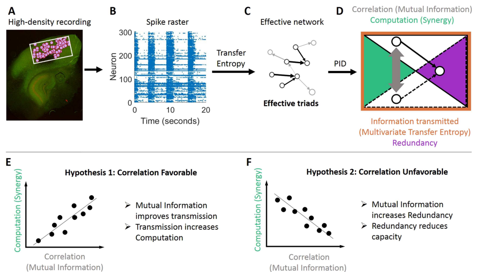
Figure 1. Methodological approach taken to ask if correlated activity is favorable or unfavorable for synergistic processing in organotypic cultures of mouse cortex. (A) Hour-long recordings of spiking activity were collected in vitro from organotypic cultures of mouse somatosensory cortex. (B) Spike sorting yielded spike trains of hundreds of well-isolated individual neurons. (C) Effective connectivity between neurons was determined by quantifying transfer entropy between spike trains. The resulting effective networks were analyzed to identify all effective triads consisting of two effective connections to a common receiver. (D) For each triad, we quantified how correlated the activity of the senders was with mutual information (gray arrow) and decomposed the total information transmitted to the receiver (measured via multivariate transfer entropy, orange perimeter) into redundancy and synergy components (via partial information decomposition, indicated with purple and green areas, respectively). (E and F) We sought to differentiate between two alternate hypotheses. (E) Predicted relationship between mutual information and synergy if correlated activity is favorable for computation. (F) Predicted relationship between mutual information and synergy if correlated activity is unfavorable for computation.
