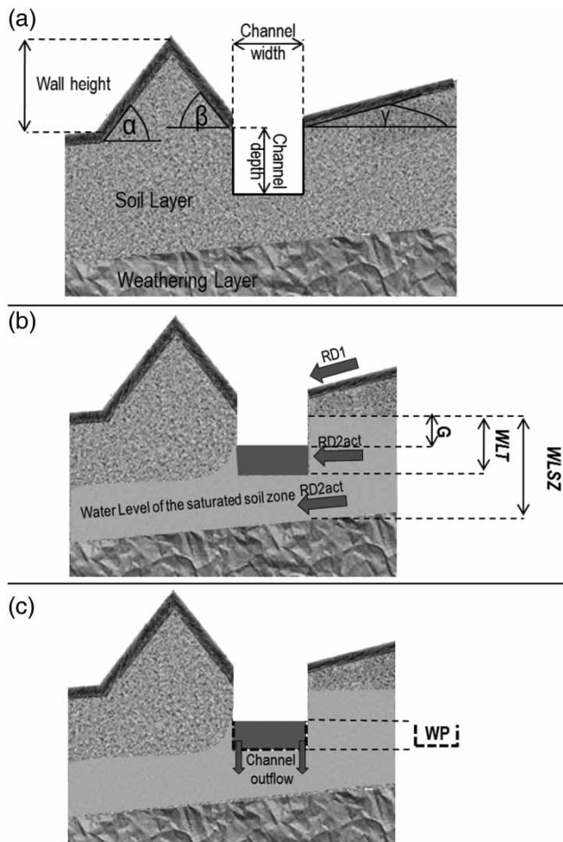
Figure 4 | (a) Simplified profile cross section of a contour bank segment and the parameters used for contour bank storage estimation. (b) Main processes of water movement within the contour bank and interaction between the contour bank storage, the runoff components of surface runoff (RD1) and actual interflow (RD2act), and the gradient (G). (c) Simplified channel outflow in dependency of the wetted perimeter (WP) between the actual water level within the trench (WLT) and the surrounding actual water level of the intermediately saturated soil zone (WLSZ).
