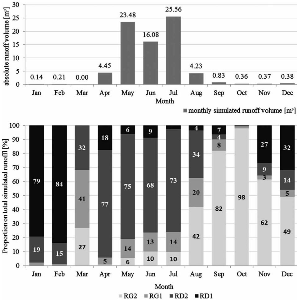
Figure 6 | Monthly simulated runoff at the catchment outlet (top) and relative proportion of single simulated runoff components on total monthly runoff volume (bottom) within the year 1990.
