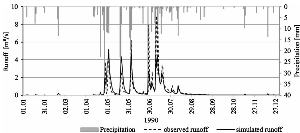
Figure 5 | Rainfall, and observed and simulated daily runoff of the Sandspruit basin for the year 1990.
