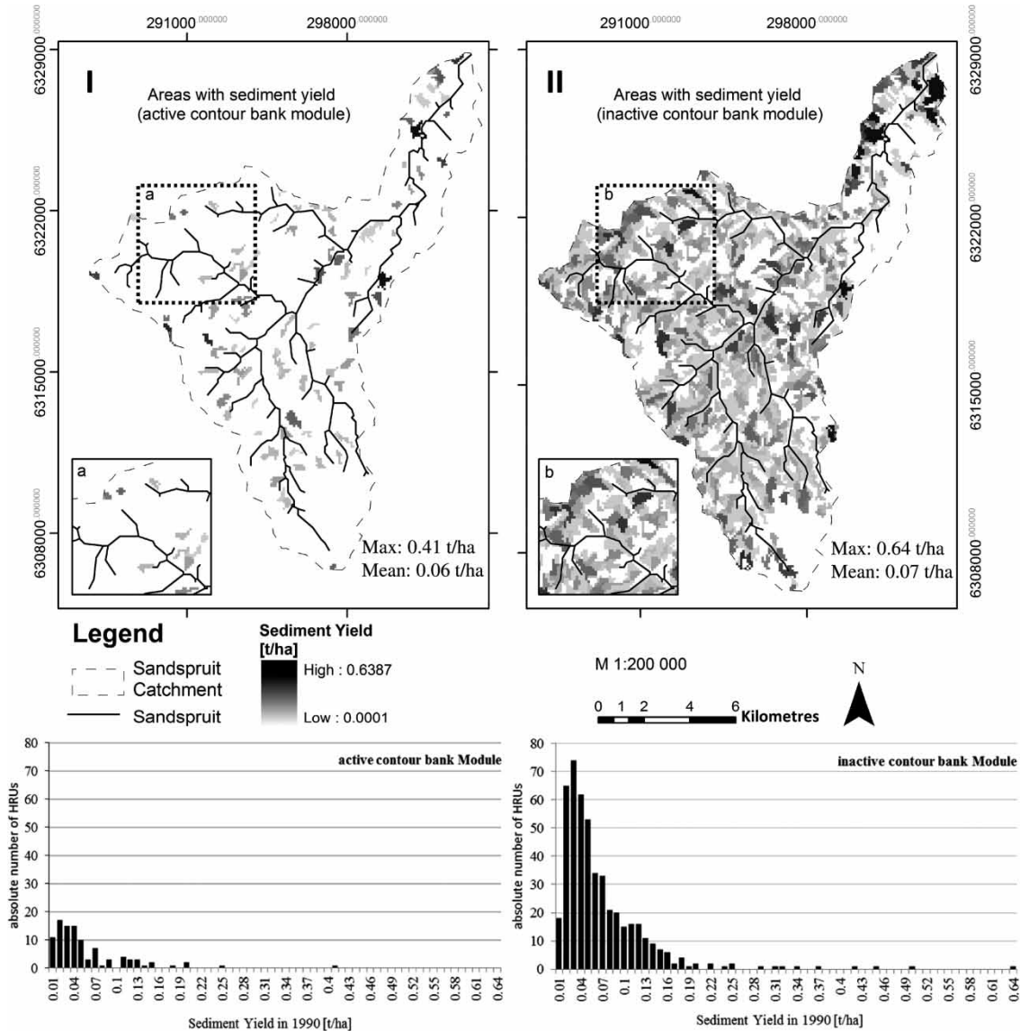
Figure 9 | Modelled sediment yield using the (I) active contour bank module and (II) no contour bank module. Top: spatial distribution of areas with simulated sediment yield. Bottom: statistical distribution of HRUs with simulated sediment yield.
