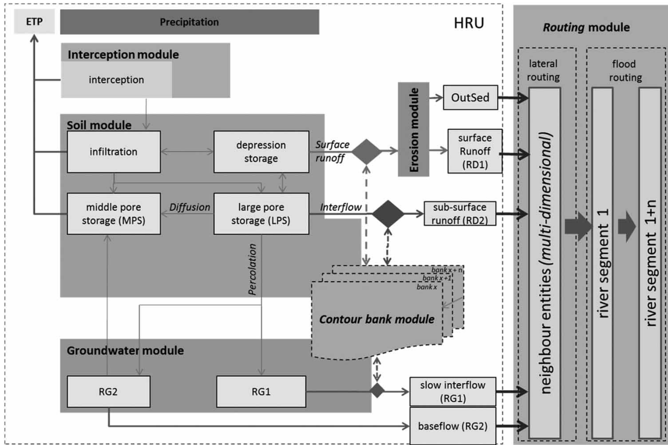
Figure 3 | Concept of the J2000 hydrological model used for the presented study (modified after Krause 2001, 2002).
