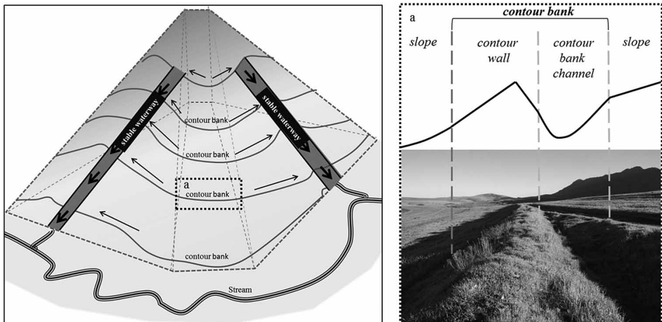
Figure 1 | Simplified impression of contour banks along a slope and waterway layout.
