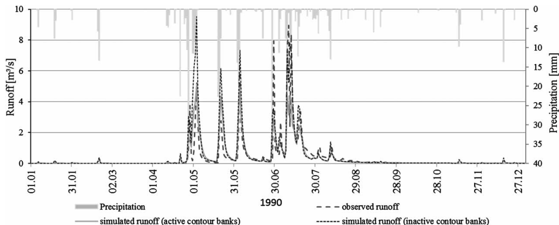
Figure 8 | Rainfall, and observed and simulated daily runoff with active and inactive contour bank module of the Sandspruit basin for the year 1990.
