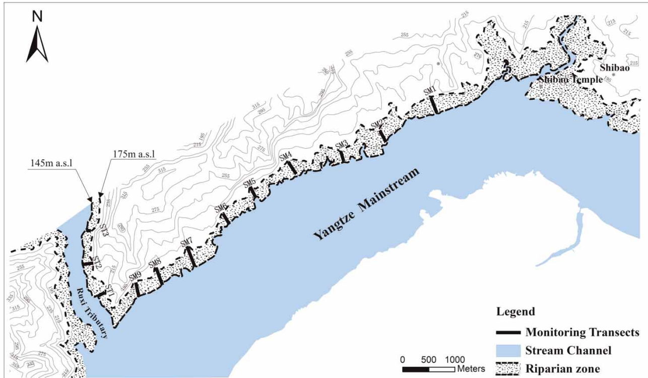
Figure 2 | Schematic representation of selected soil erosion monitoring transects along the mainstream and Ruxi tributary.
