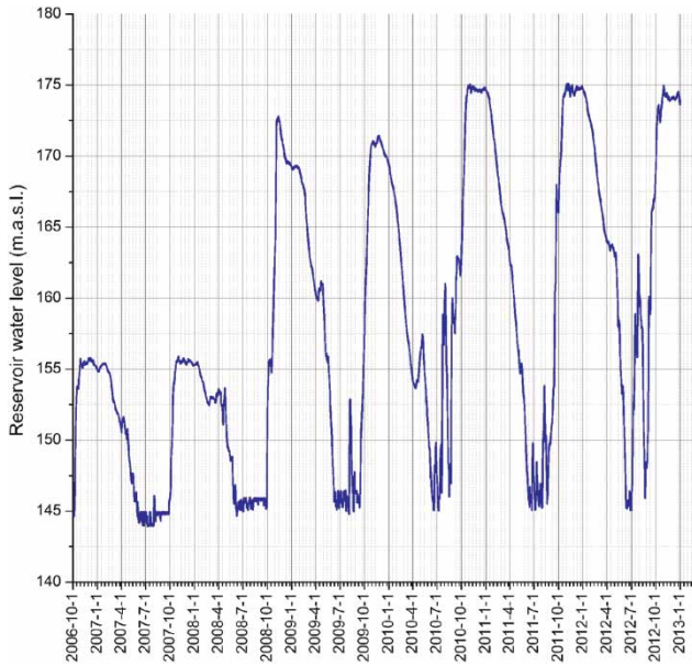
Figure 3 | Water level fluctuating schedule in the riparian zone of the TGR during 2006–2012.
