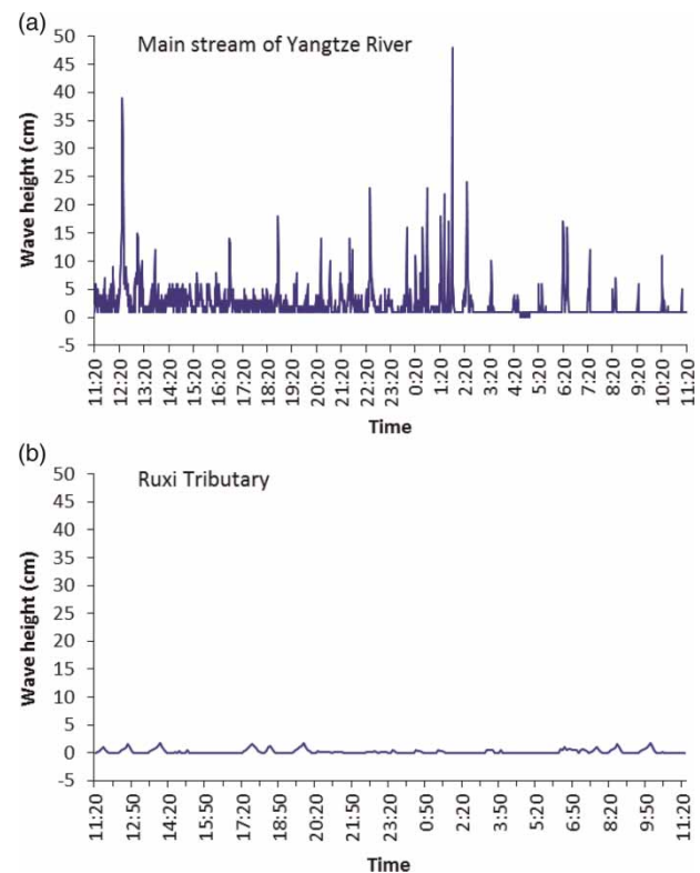
Figure 6 | Monitored wave heights in the Yangtze mainstream and the Ruxi tributary.
