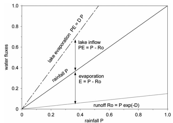
Figure 2 | Water fluxes derived from the minimalist model of terminal Lake Qinghai with lake area ratio A \sim 0.145 dependent dryness ratio, D \sim 1.9 . (i) Land water fluxes comprise evaporation E and runoff Ro adding up to precipitation P (main diagonal). (ii) Lake evaporation PE = E_{\text{lake}} = DP for D \geq 1 exceeds the main diagonal (1:1) because it is balancing the sum of precipitation P (main diagonal) and inflow ( Ri ) from the catchment, Ro_{\text{lake}} = P - PE = (1 - D)P < 0 .
