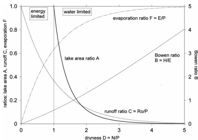
Figure 1 | Minimalist model of terminal lakes in a climate state diagram: dryness ratio dependent climate variables are the lake area ratio A , the Bowen ratio B , the runoff ratio C and evaporation ratio F .
