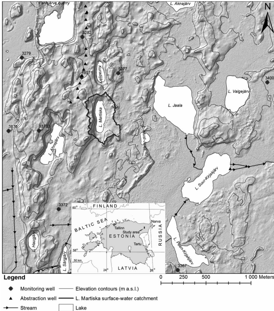
Figure 1 | Location and topography of the surface-water catchment of L. Martiska with location of wells used for groundwater abstraction and water level monitoring (the digital elevation model was created according to year 2009 LIDAR-points obtained from the Estonian Land Board).
