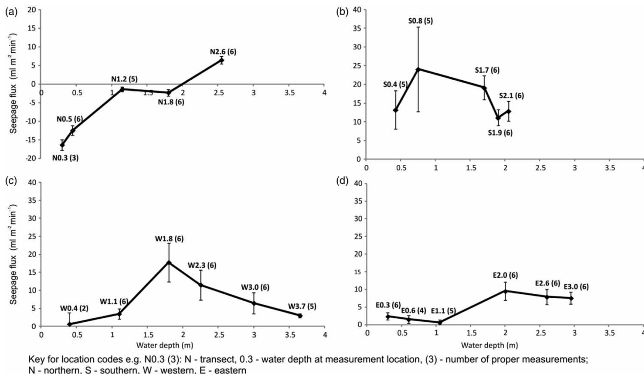
Figure 3 | Seepage fluxes at the measurement locations on the (a) northern, (b) southern, (c) western and (d) eastern transect.
