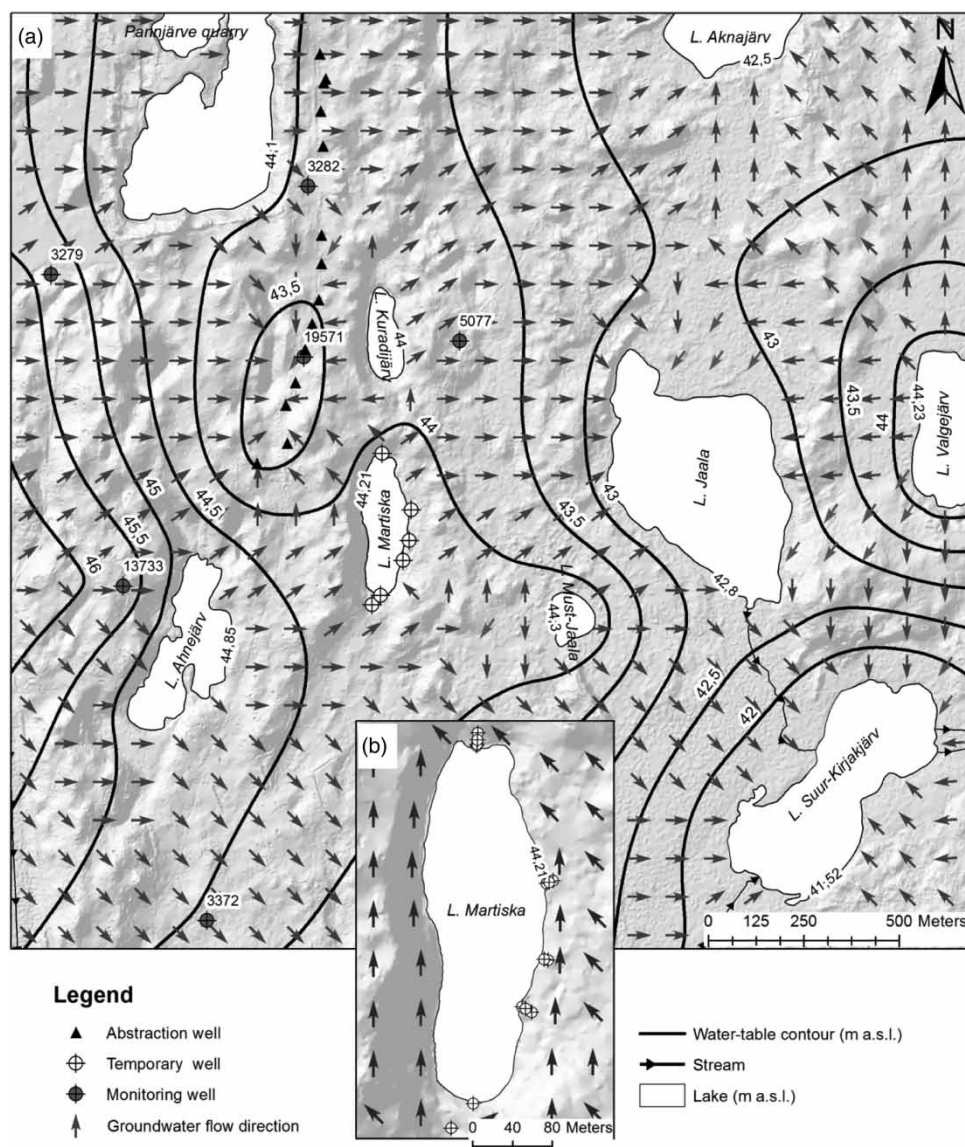
Figure 5 | (a) Piezometric map and groundwater flow directions in the central part of the Kurtna Lake District in June 2012, interpolated according to water levels from temporary and permanent wells and lake levels; (b) groundwater flow directions around L. Martiska in June 2012, interpolated according to water levels from temporary wells and the lake level (the digital elevation model was created according to year 2009 LIDAR-points obtained from the Estonian Land Board).
