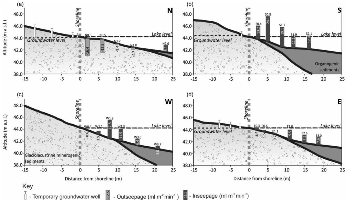
Figure 4 | Seepage direction and rates on the (a) northern (N), (b) southern (S), (c) western (W) and (d) eastern (E) transects of L. Martiska in June 2012. The heights of the columns indicate seepage rate at that location. The numbers in the measurement location codes, e.g. N0.3, indicate water depth at that location in meters. Seepage direction and rates are shown in the context of onshore groundwater level and characteristics of the measurement location – sediment type (minerogenic vs. organogenic) and organic sediment thickness.
