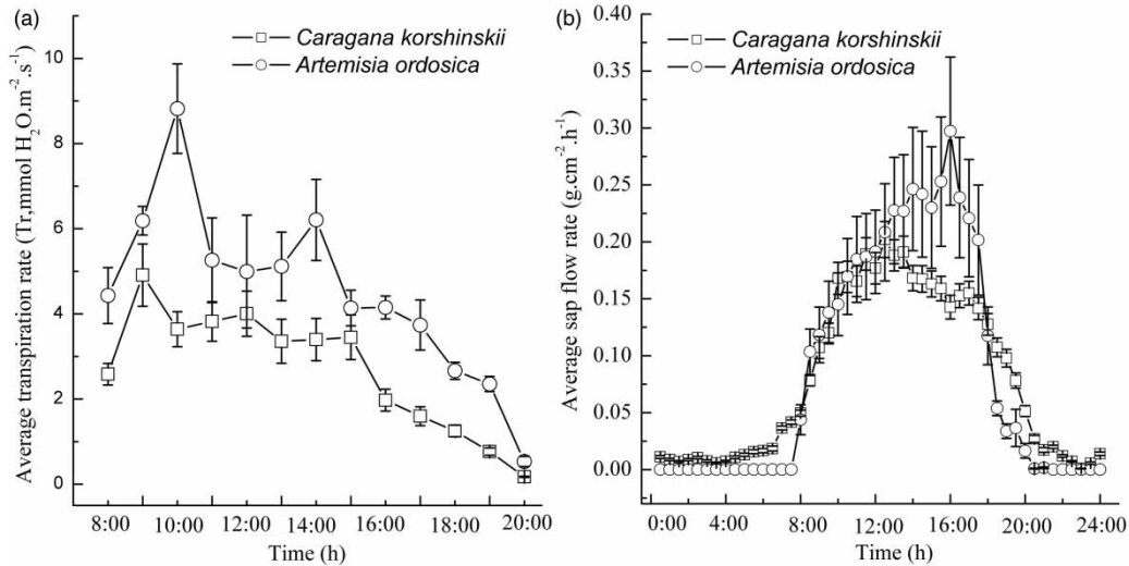
Figure 2 | Diurnal course of transpiration rate \text{Tr} (a) and the sap flow rate (b) in C. korshinskii and A. ordosica during the experimental period (April 2008–October 2012).
