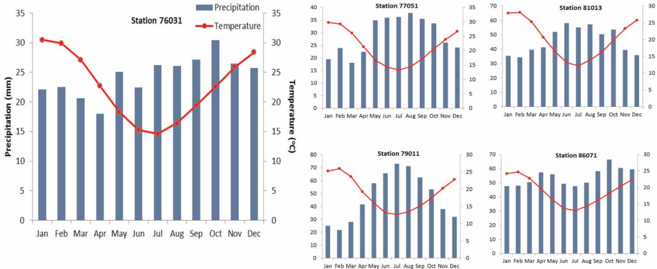
Figure 2 | Mean monthly precipitation and temperature for all stations.
