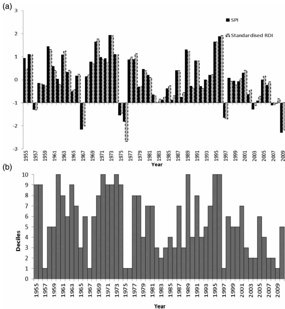
Figure 5 | Droughts identified using (a) SPI and RDI and (b) deciles on 6-month time scale for Station 86071.
