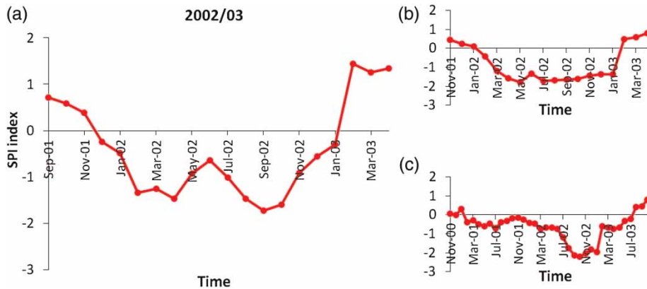
Figure 8 | Onset and end of drought for 2002–2003 on (a) 3-month, (b) 6-month and (c) 12-month time scales for Station 77051.
