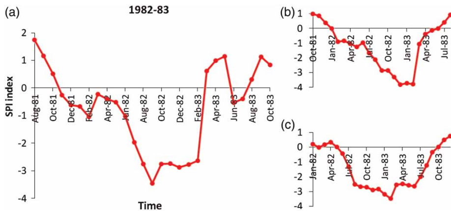
Figure 7 | Onset and end of drought obtained from the SPI on (a) 3-month, (b) 6-month and (c) 12-month time scales for Station 77051.
