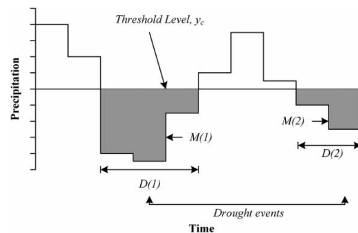
Figure 3 | Characteristics of local drought events with the ToR (Paulo & Pereira 2006).
