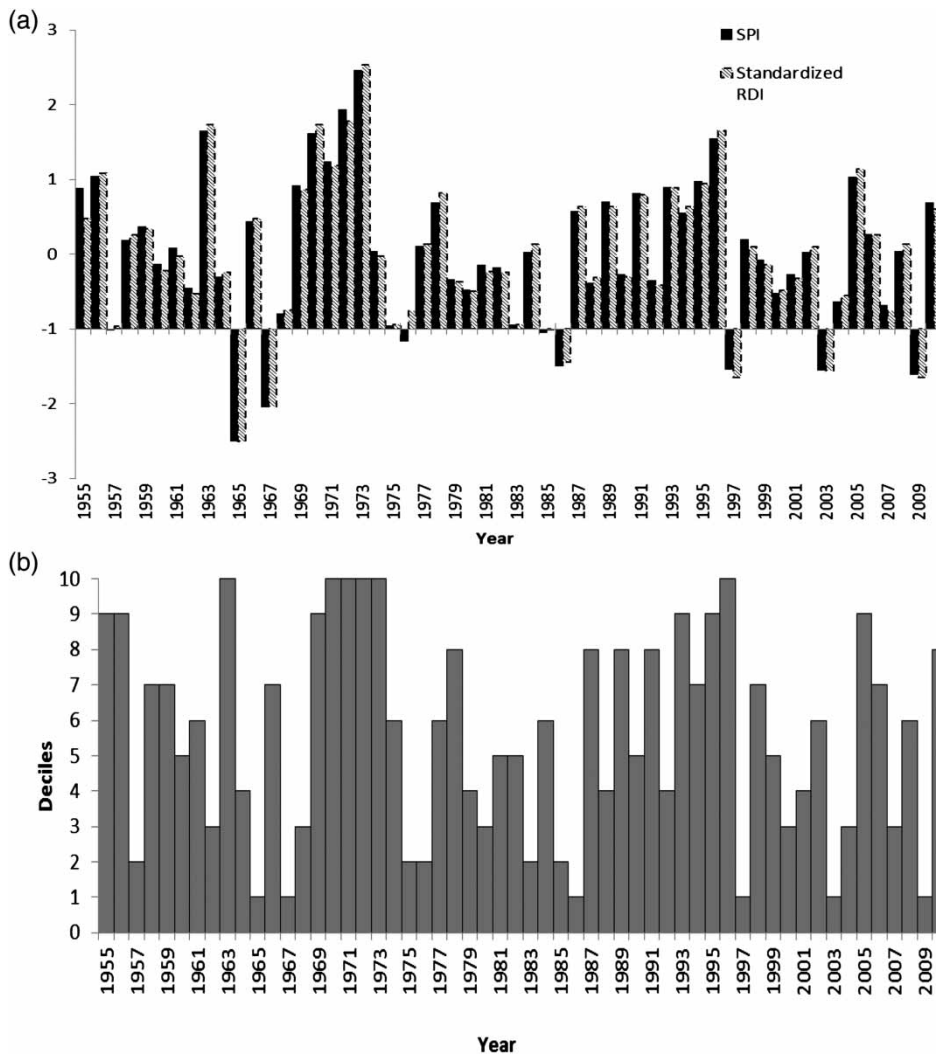
Figure 4 | Droughts identified using (a) SPI and RDI and (b) deciles on 3-month time scale for Station 86071.
