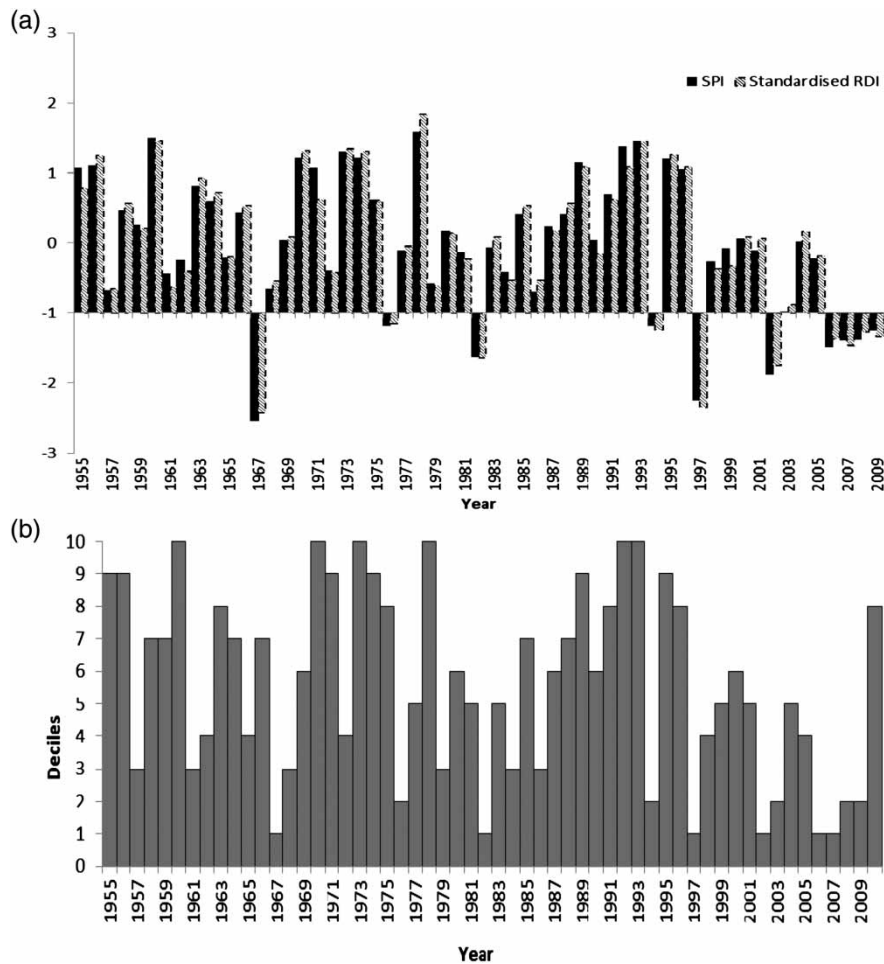
Figure 6 | Droughts identified using (a) SPI and RDI and (b) deciles on 12-month time scale for Station 86071.
