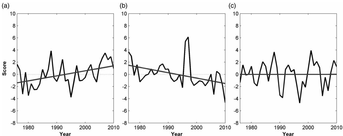
Figure 4 | Time series of annual runoff PC scores for the northern region (a), middle region (b), and southern region (c).
