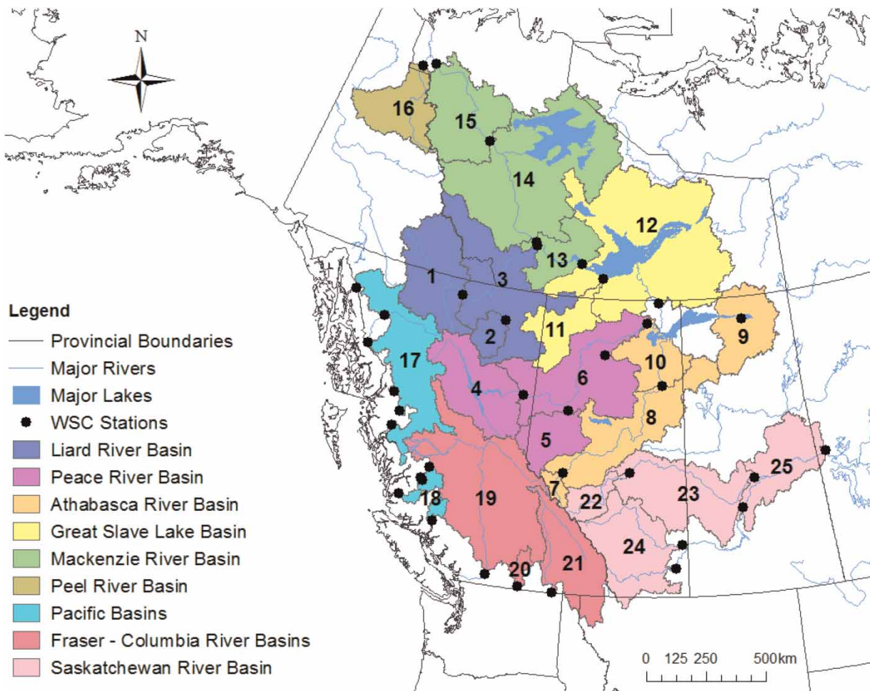
Figure 1 | Map of the study area showing delineation of the watersheds.
