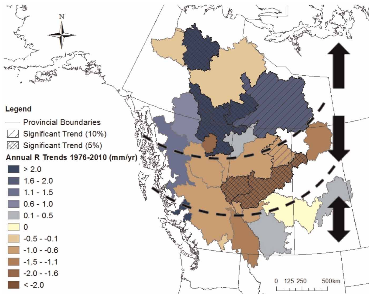
Figure 2 | Annual runoff trend magnitudes.
