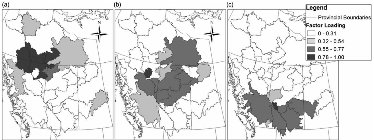
Figure 3 | Annual runoff PC loadings for each watershed for the PC defining the northern region (a), middle region (b), and southern region (c).
