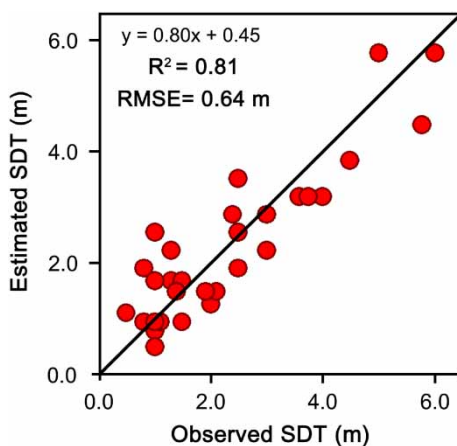
Figure 3 | Scatter plot of Landsat-estimated and observed SDT with 1:1 fit line.
