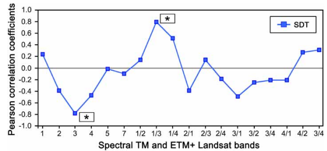
Figure 2 | Pearson correlation coefficients between SDT versus Landsat spectral bands and band ratios. Asterisks represent the spectral bands retained by the step-wise multiple regression analysis ( p < 0.05 ).
