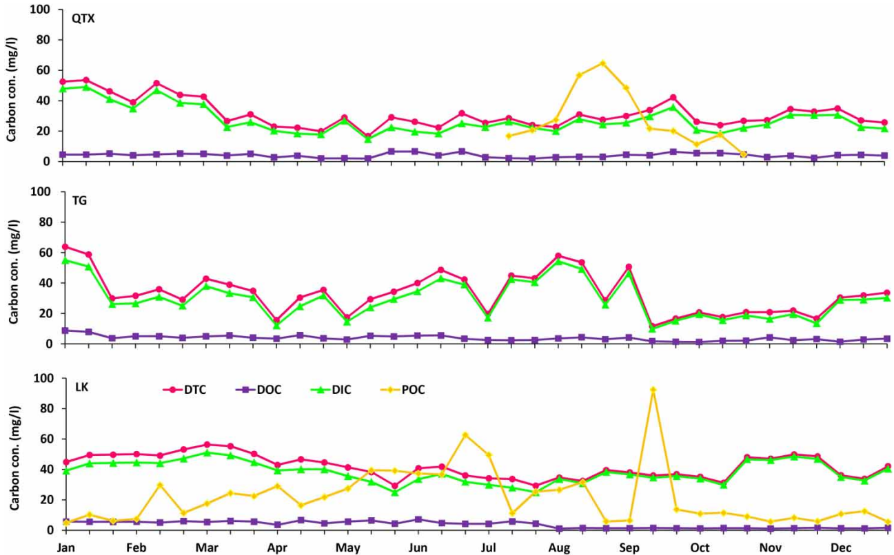
Figure 3 | Seasonal variations of carbon concentrations in different forms at QTX (upstream), TG (midstream), and LK (downstream) during 2006.
