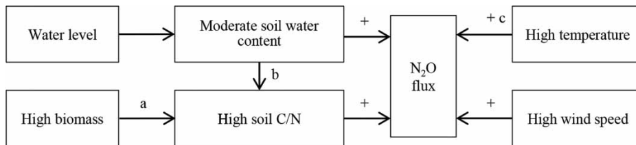
Figure 6 | Conceptual model of drivers of N_2O emission. Symbols (+) represent positive effects. (a) Plants have both positive and negative effect on soil nutrients through consumption of nutrients for growth and addition of nutrients resulting from decomposition of tissues. (b) High SWC is conducive to the accumulation of SOM. (c) In this work, we see a negative correlation between temperature and flux; we propose this uncommon correlation occurs because the positive effect of temperature on decomposition is masked by even stronger effects from SWC and nutrients.
