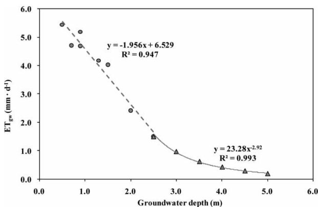
Figure 4 | Relationship between average daily ET_{gw} and groundwater depths.
