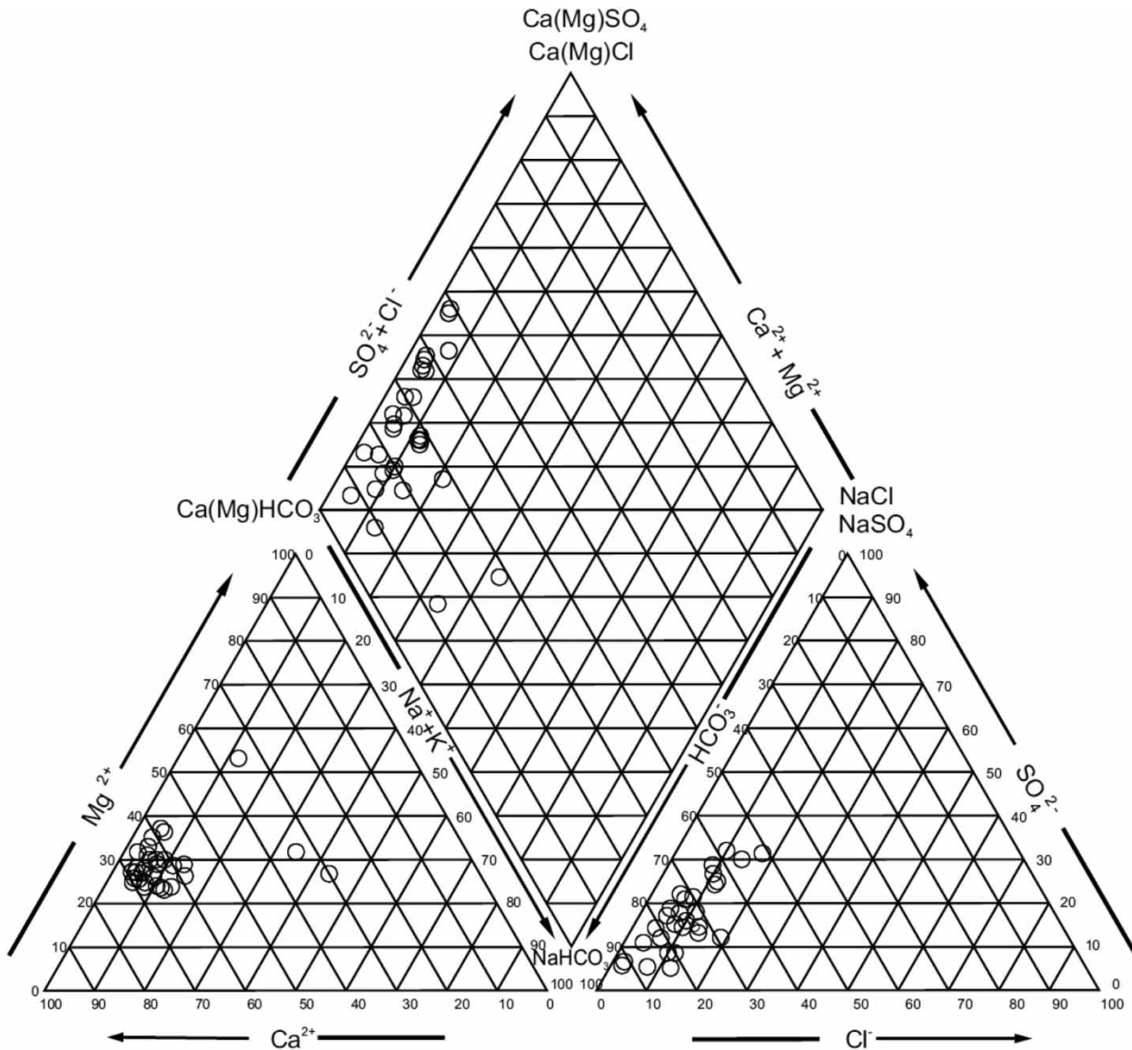
Figure 3 | Piper diagram.
