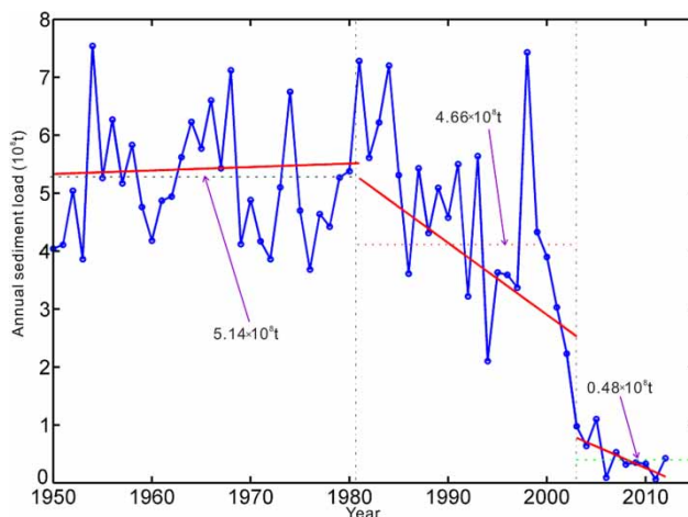
Figure 7 | Annual sediment load at Yichang station.
