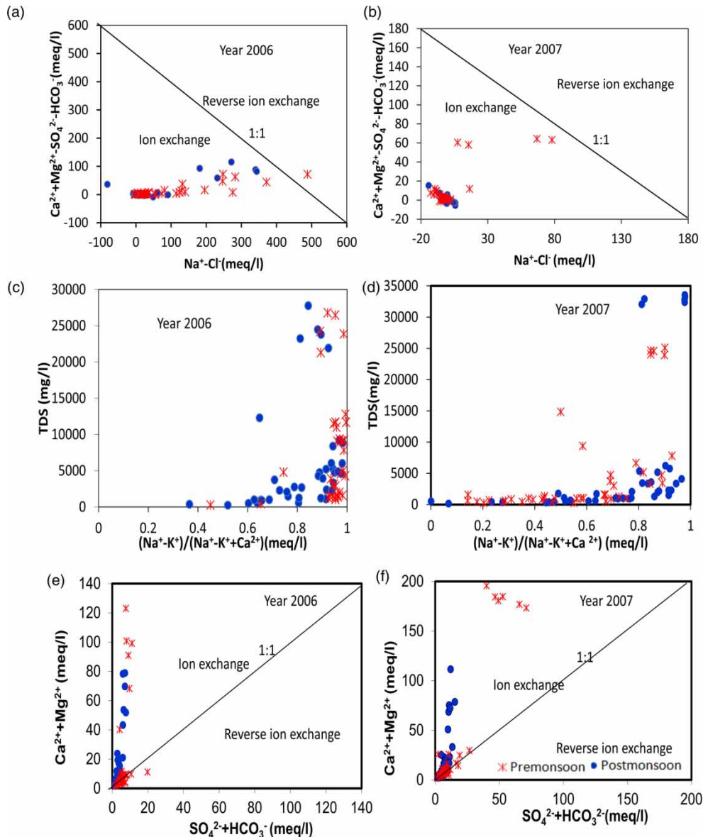
Figure 3 | X-Y diagrams illustrating relationships among the major ions and ion exchange process.
