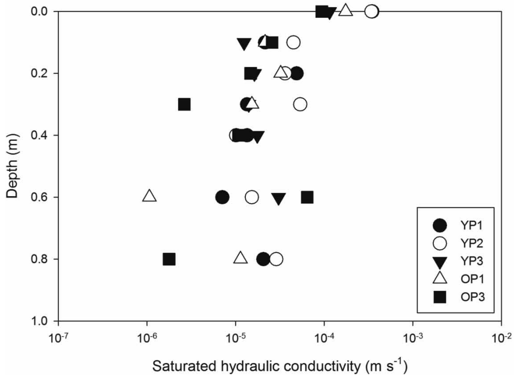
Figure 4 | Vertical profiles of saturated hydraulic conductivity ( K_s ).
