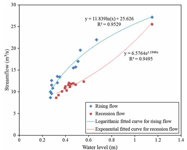
Figure 2 | Rope relation curve between discharge and water level at the catchment outlet.
